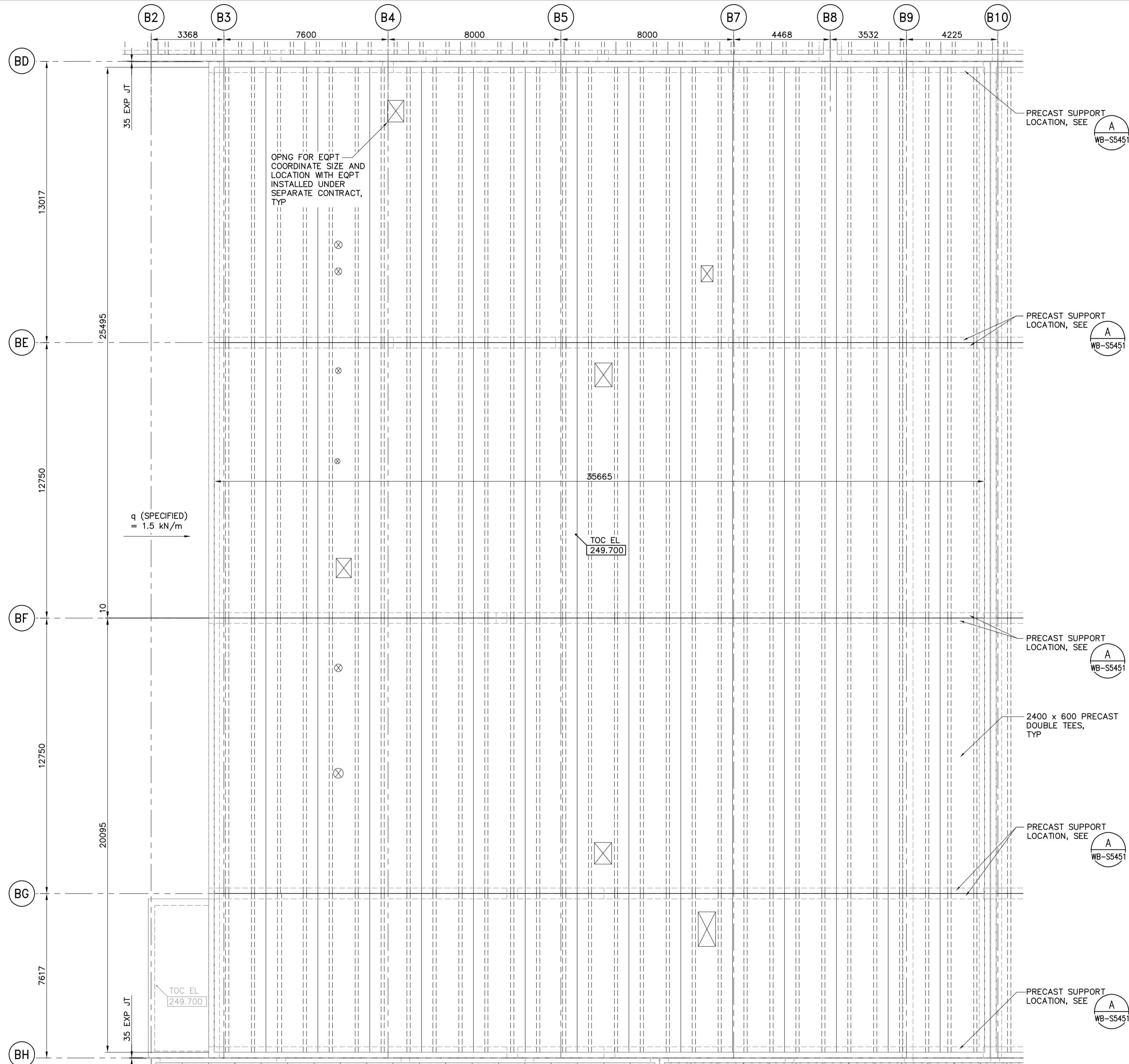
ROOF PLAN 1:100
