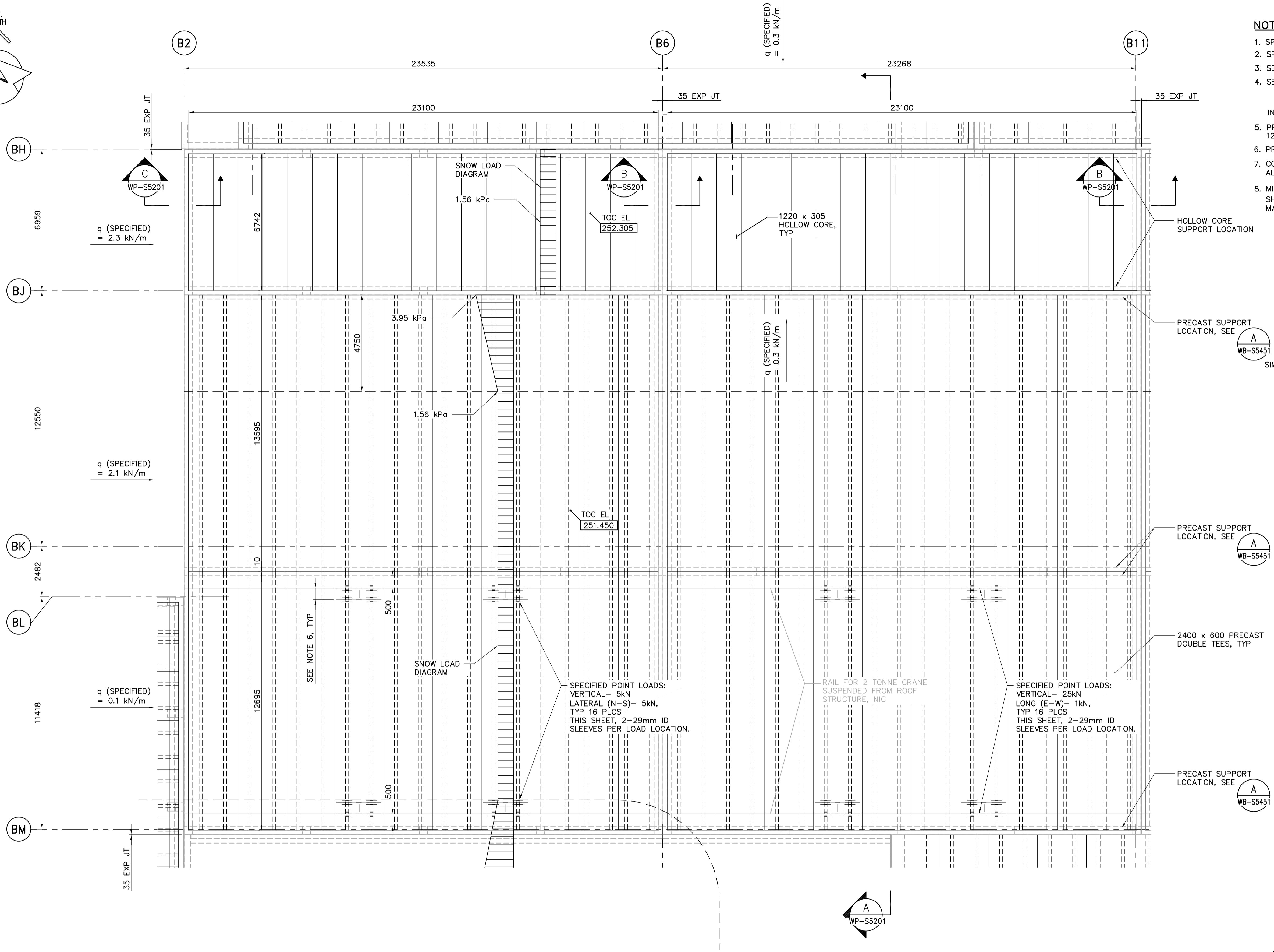
ROOF PLAN 1:100
