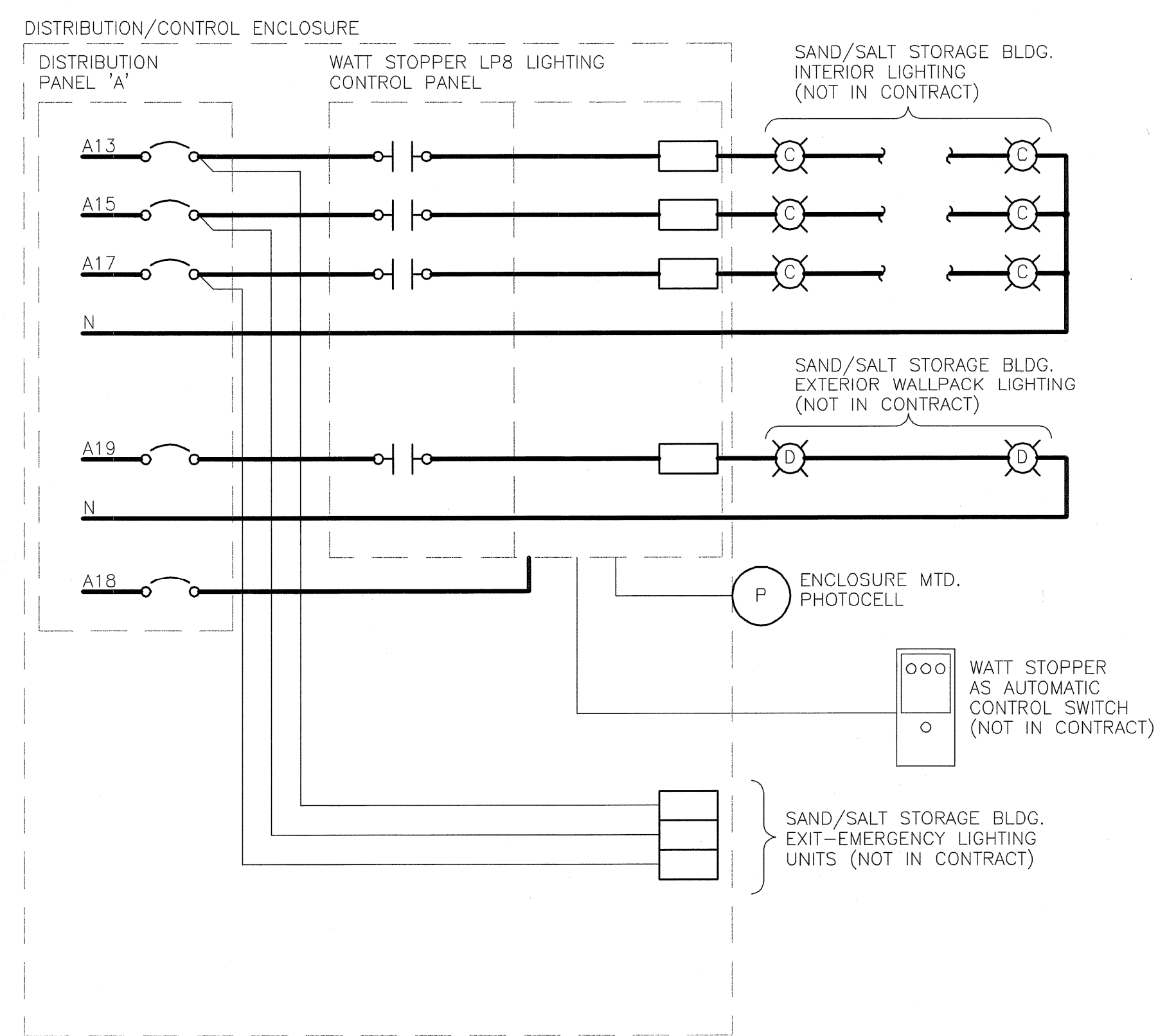
B LIGHTING CONTROL SCHEMATIC N.T.S.
