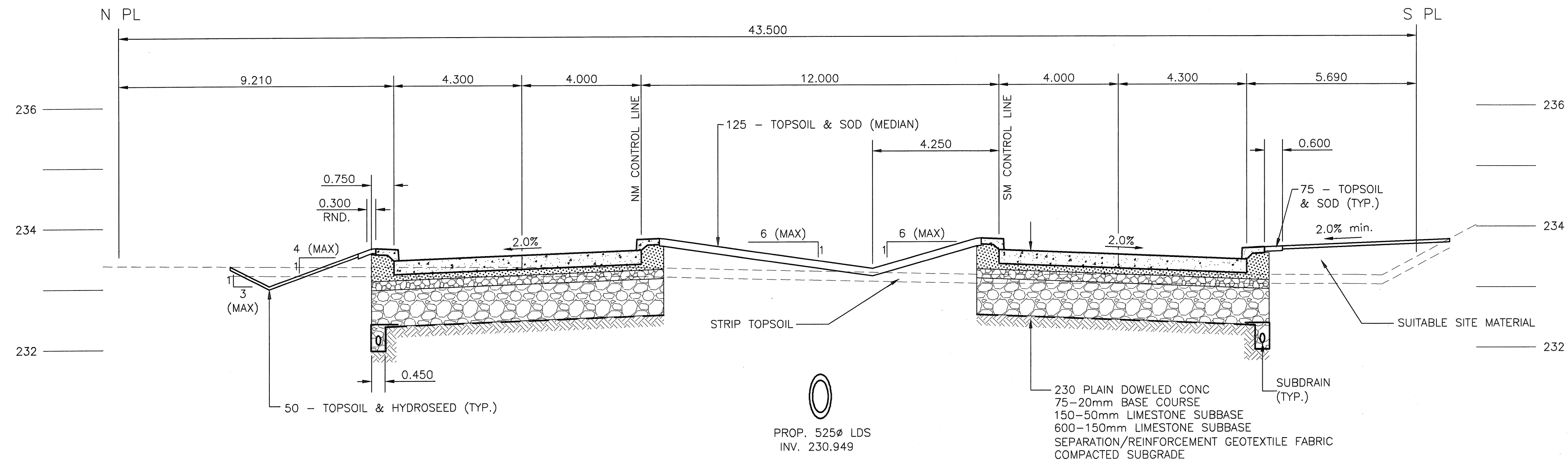
STERLING LYON PARKWAY SECTION @ STA. 2+210NM
