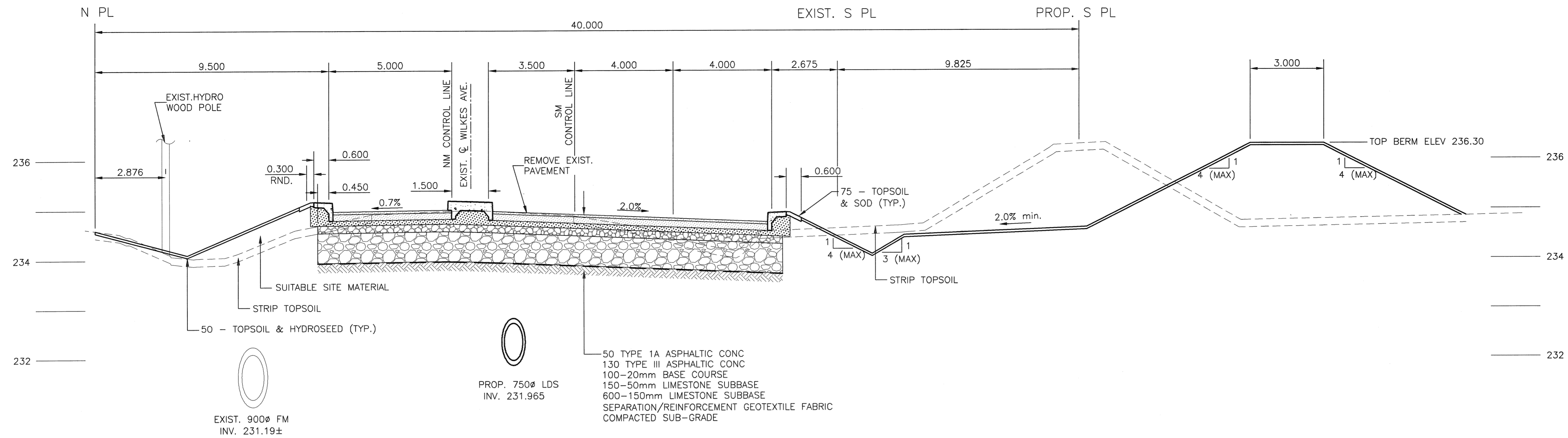
WILKES AVENUE SECTION @ STA. 0+700NM
