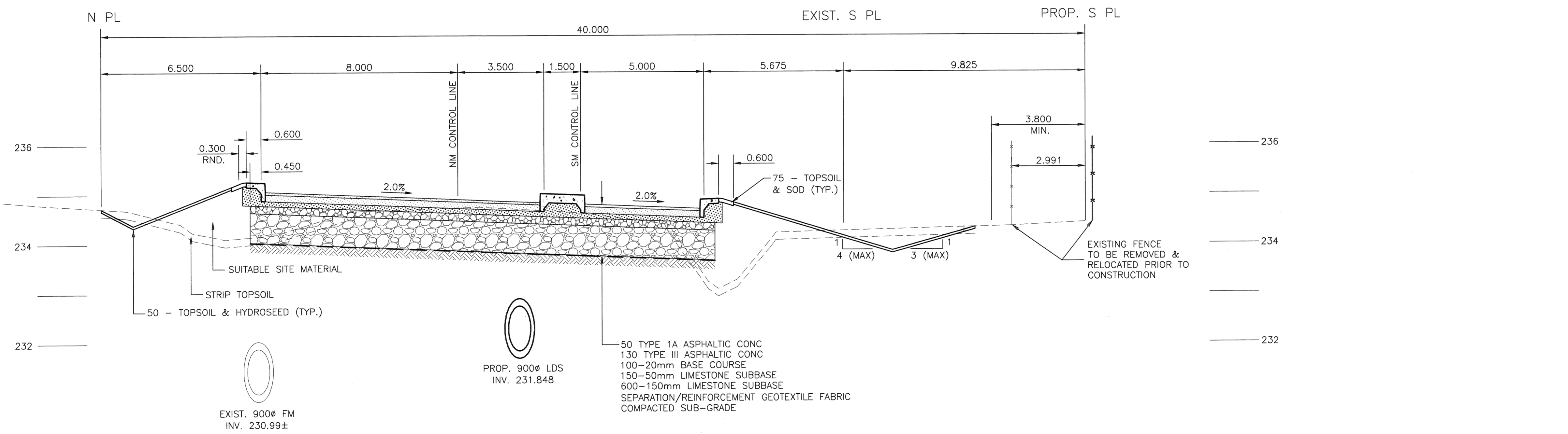
WILKES AVENUE SECTION @ STA. 0+800NM
