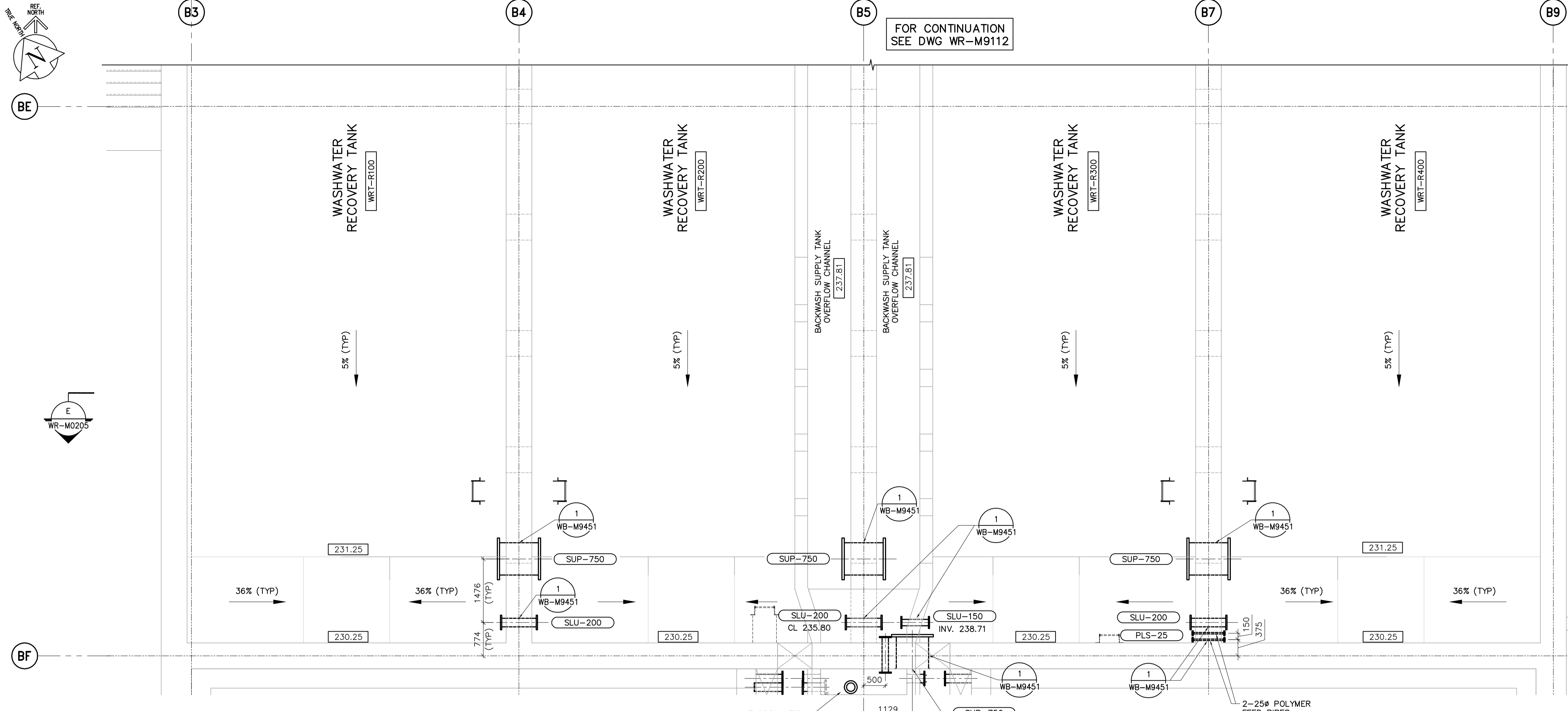
PLAN VIEW AT ELEVATION 239.000 1:50
