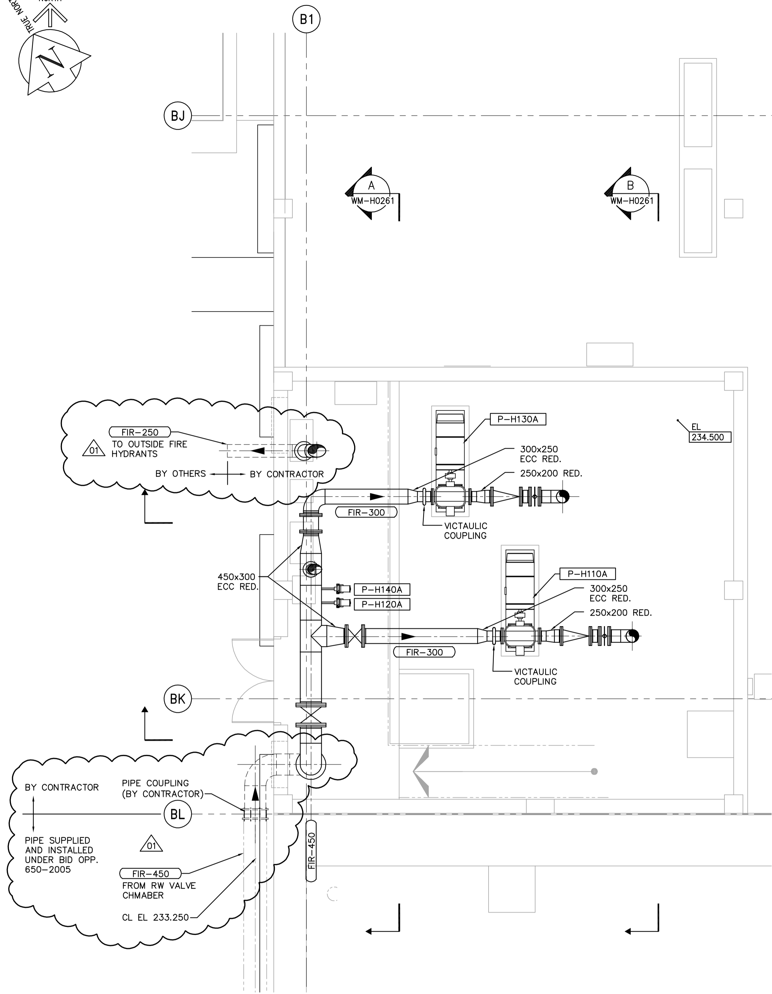
LOWER LEVEL PLAN 1:50
