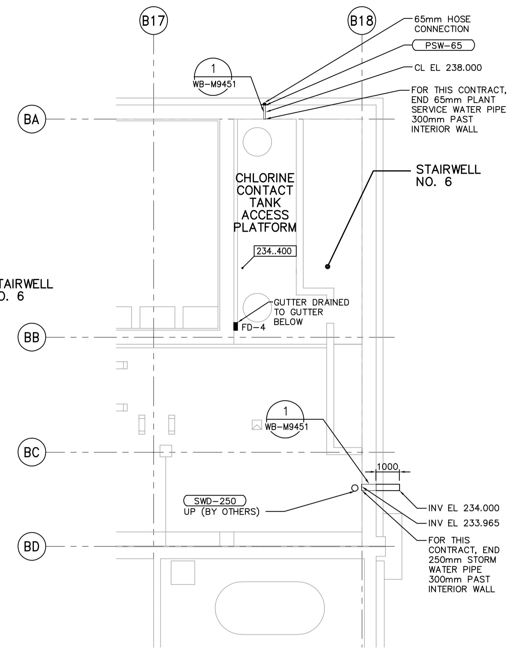
PARTIAL FIRST FLOOR PLAN 1:100
