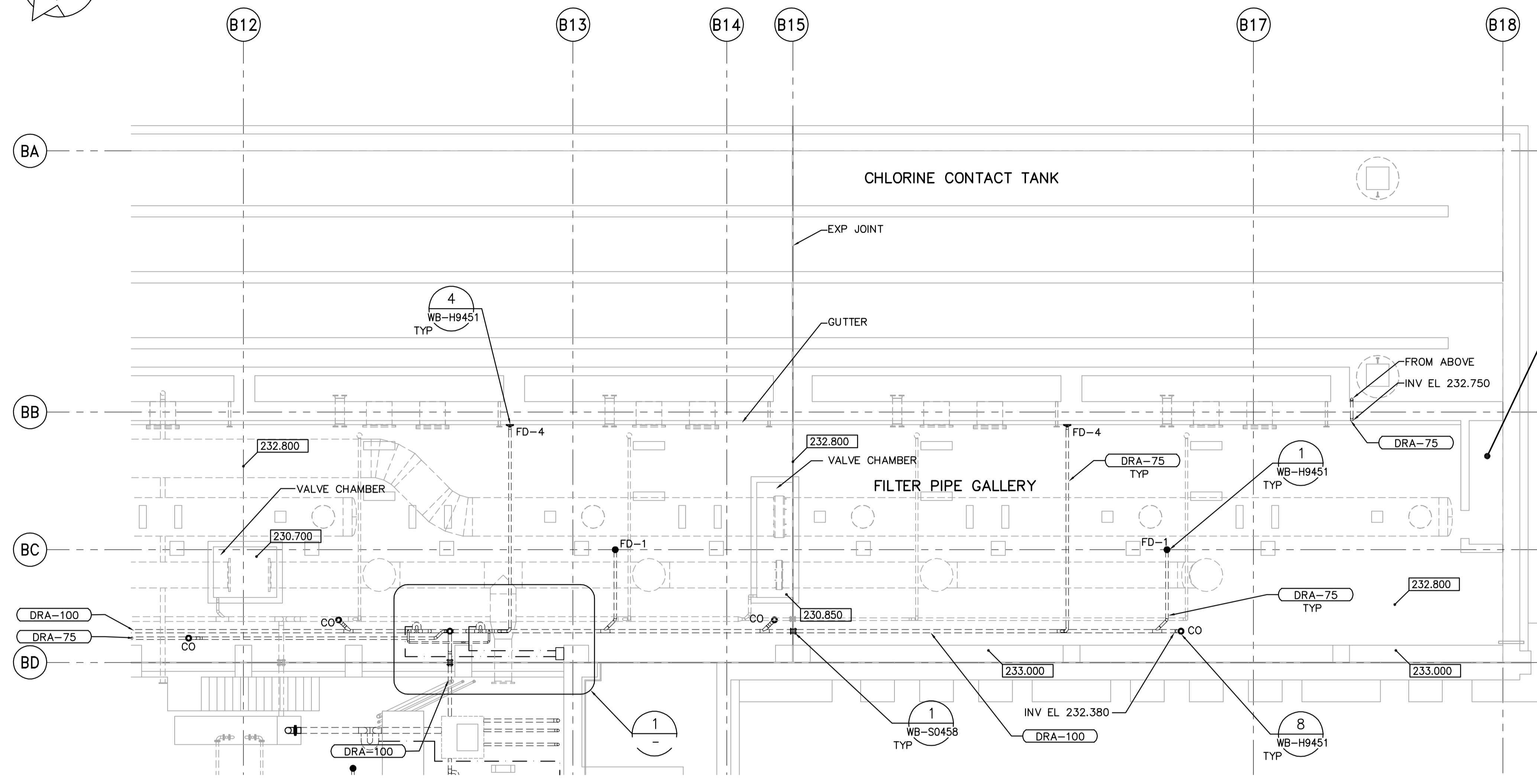
LOWER LEVEL PLAN 1:100
