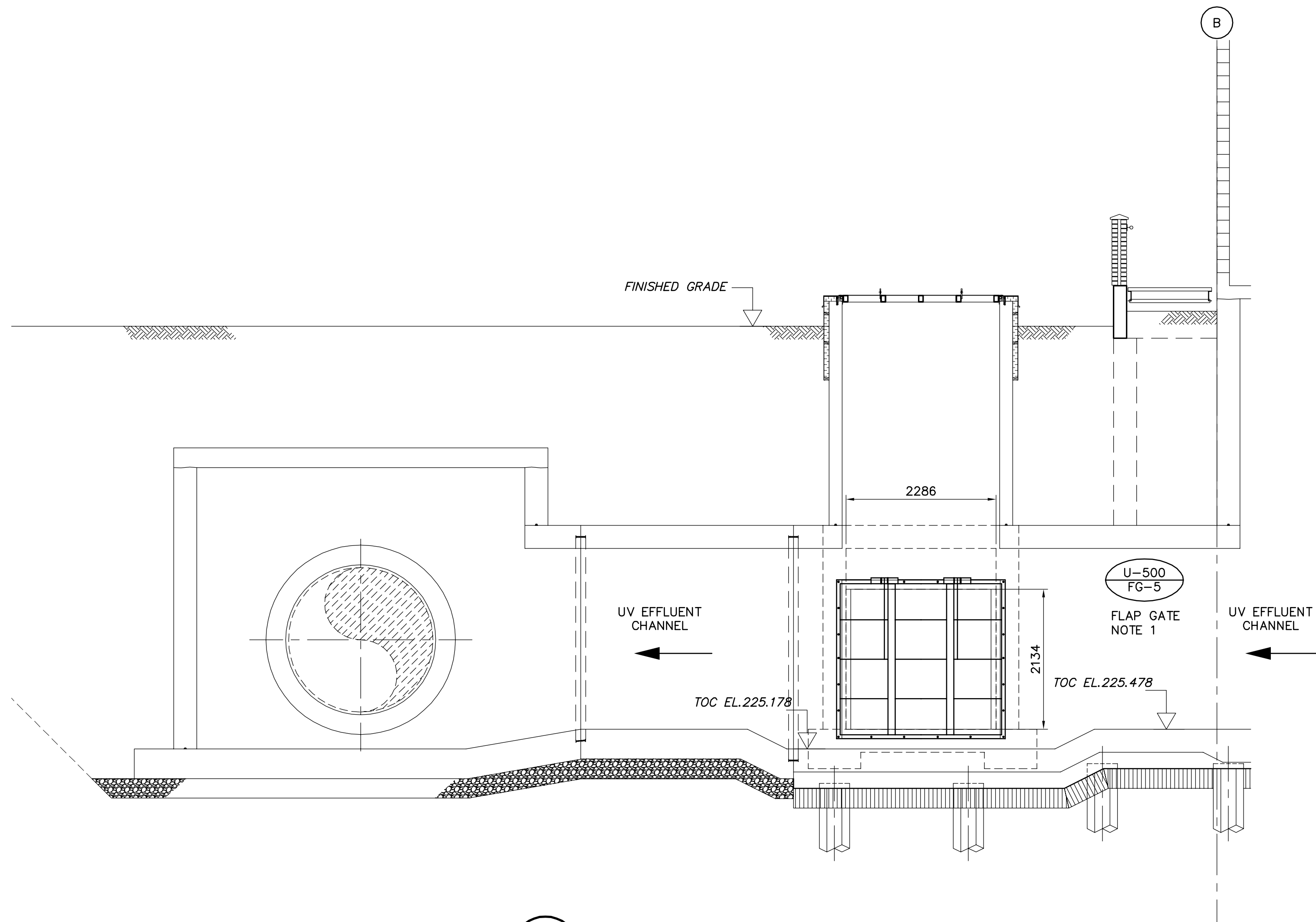
D SECTION P2.02 SCALE 1:50
