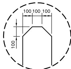
DETAIL 1 -PIER NOSE
