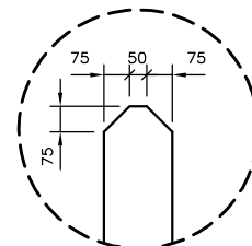
DETAIL 2 -PIER NOSE
