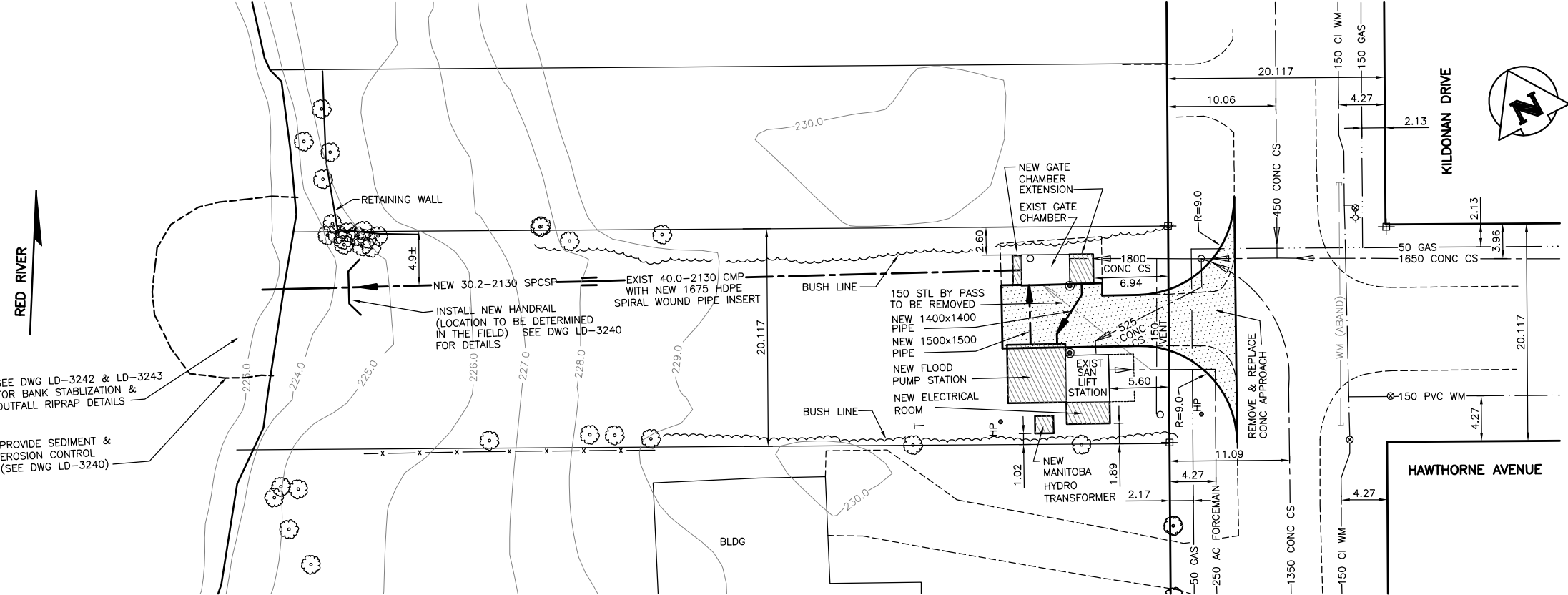
HAWTHORNE AVE OUTFALL RR-98
