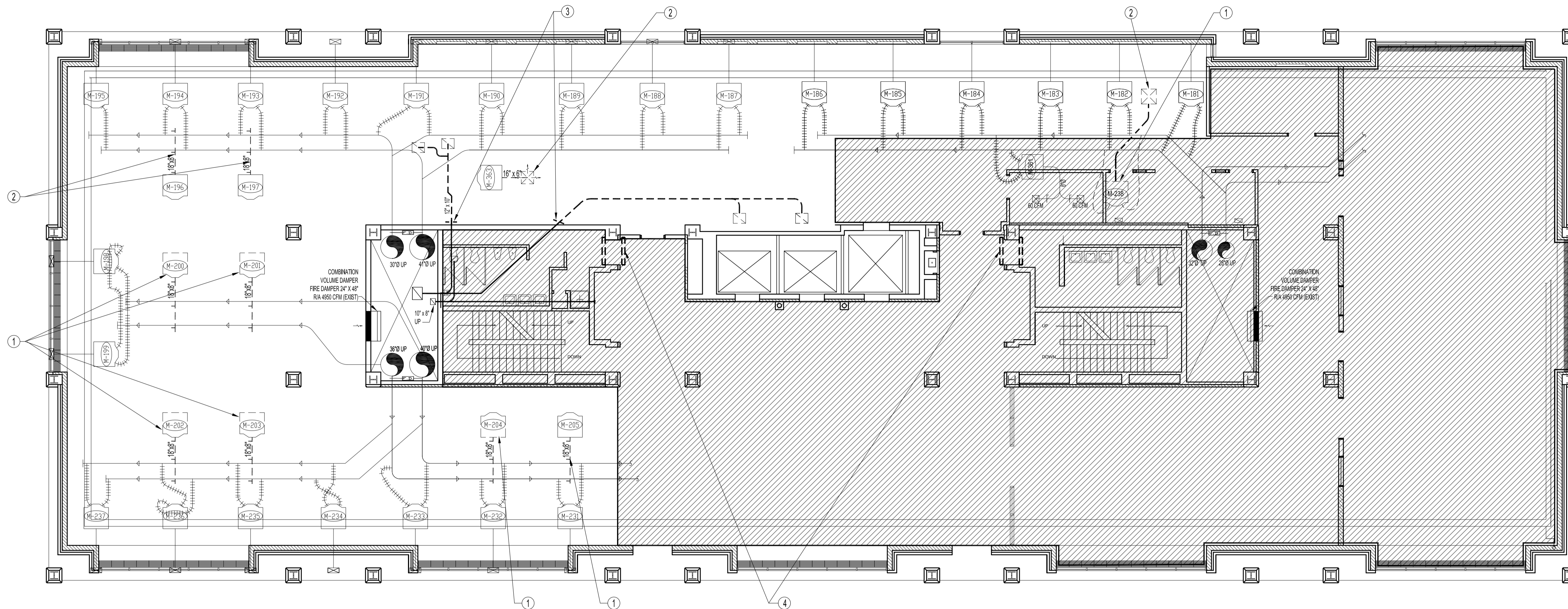
SECOND FLOOR PLAN - MECHANICAL DEMOLITION SCALE: 1/8"=1'-0"
