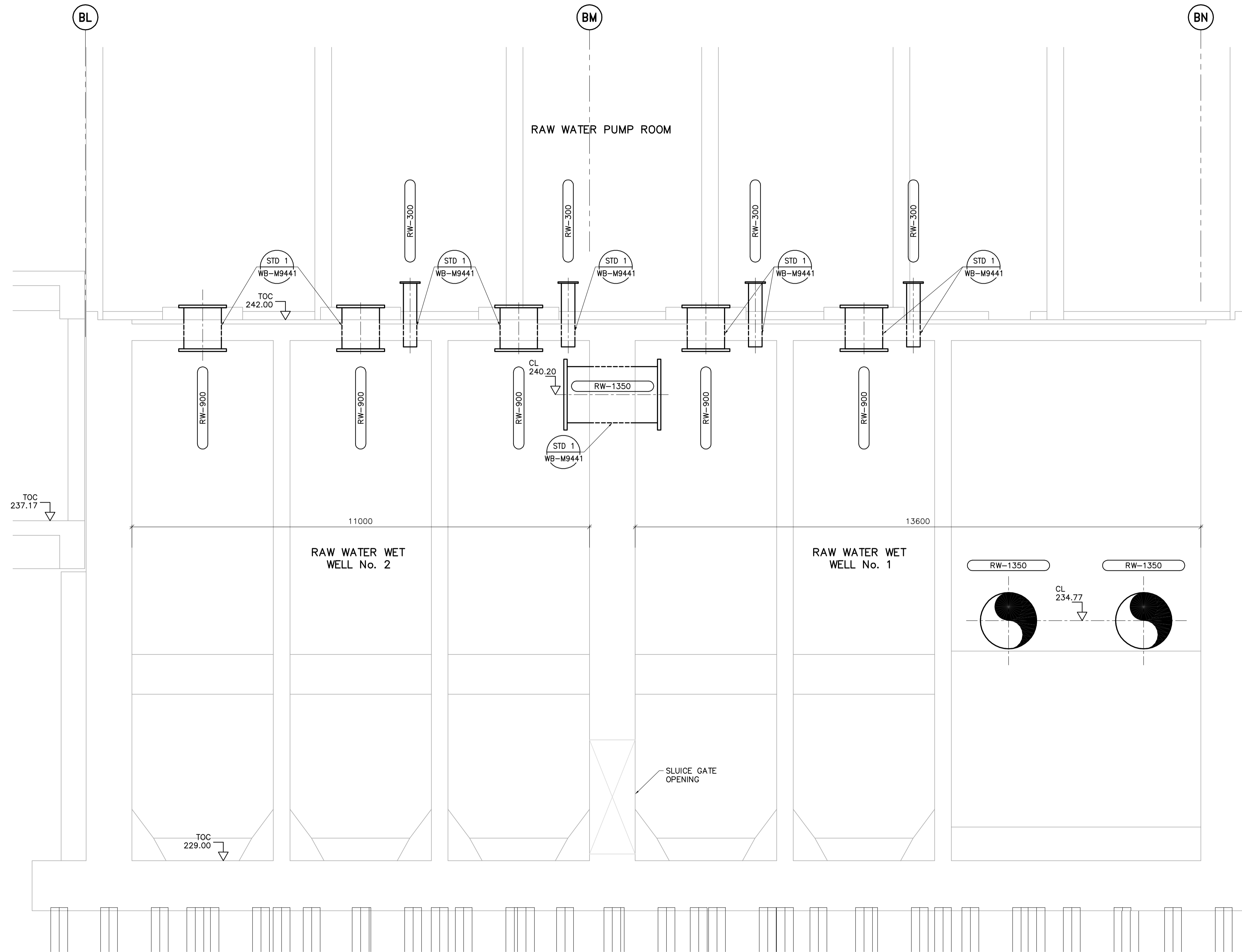
B SECTION WI-M9101 1:50
