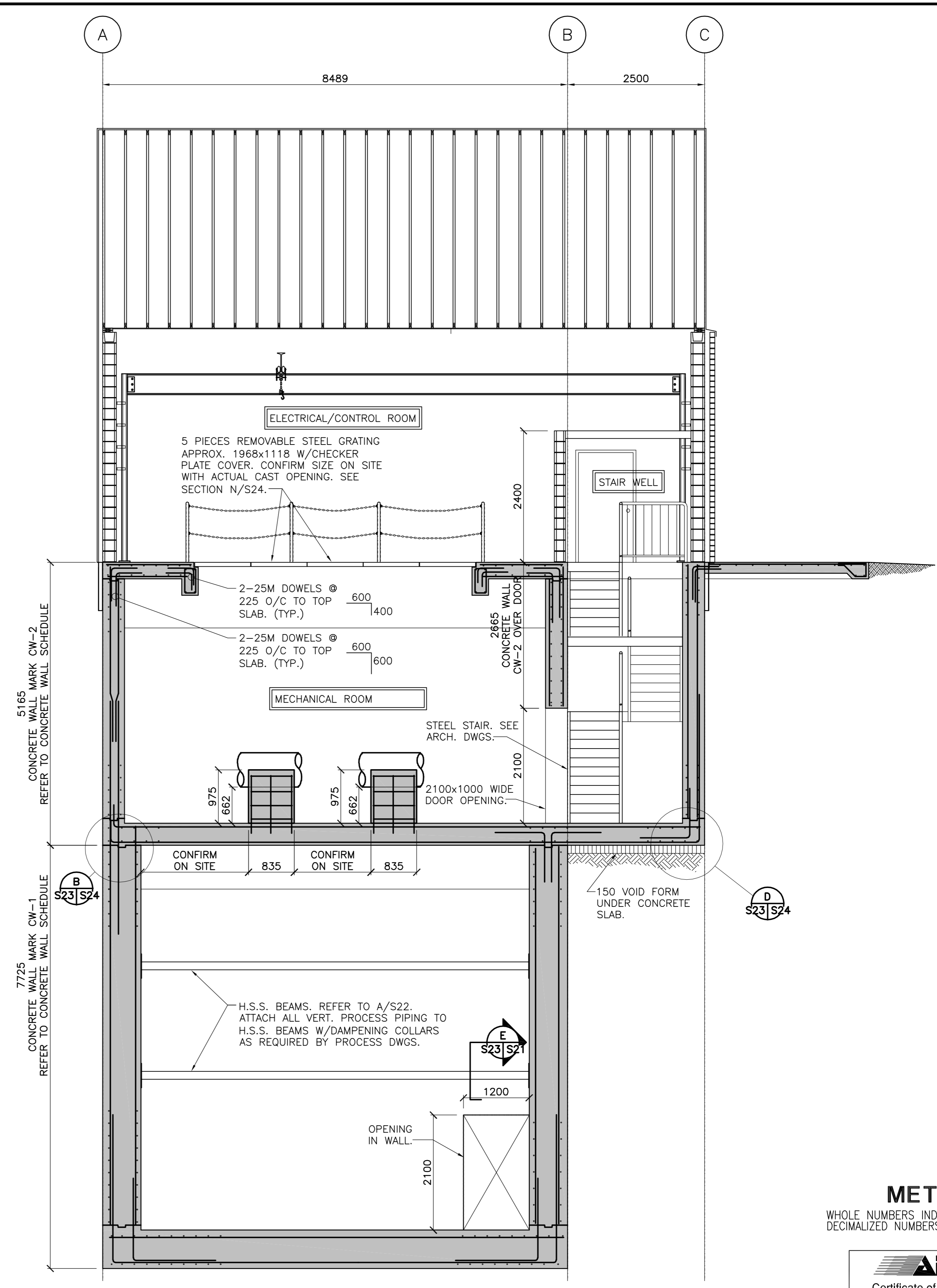
BUILDING SECTION D D S19 S23 S20 S23 1:50
