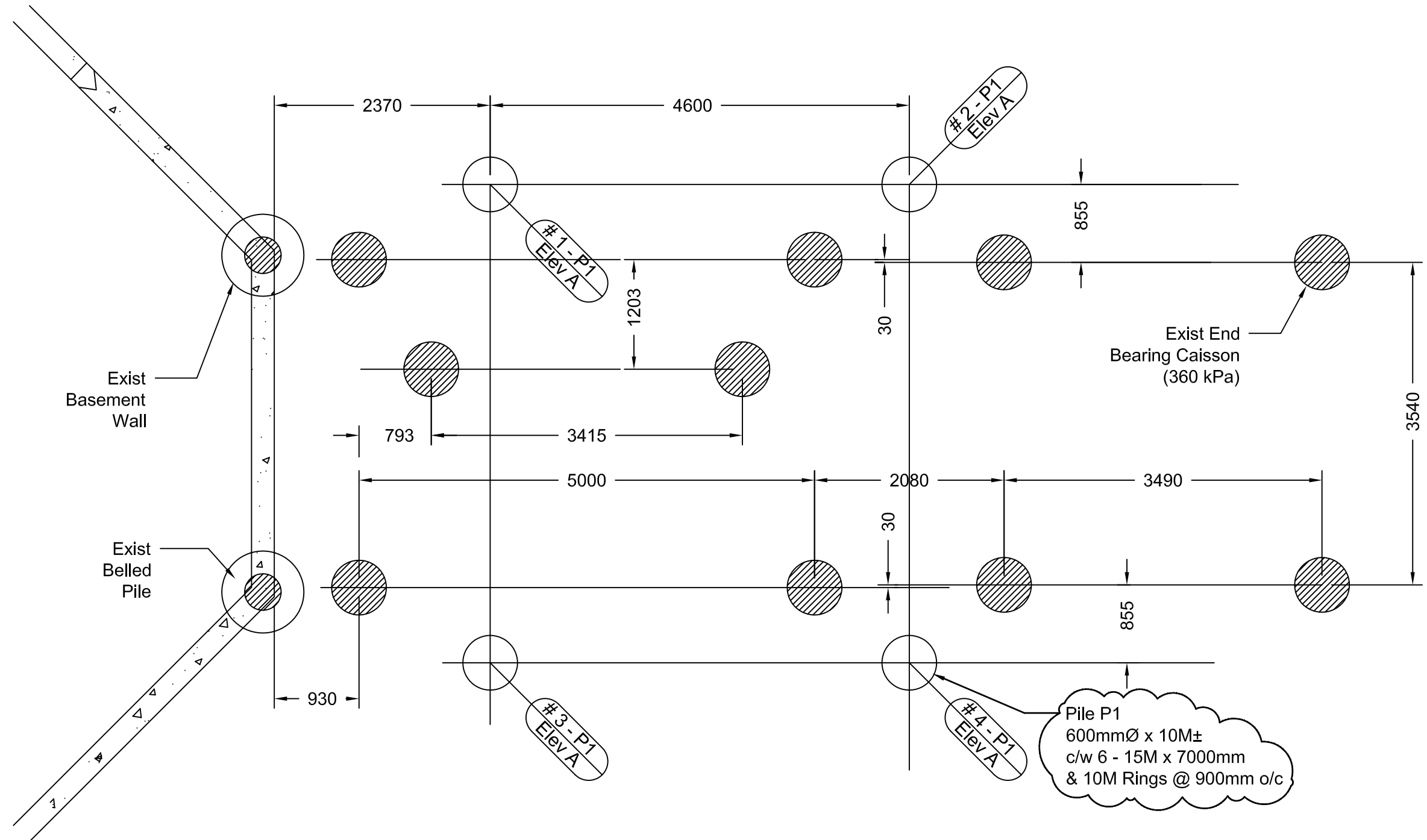
FOUNDATION PLAN SCALE 1:50
