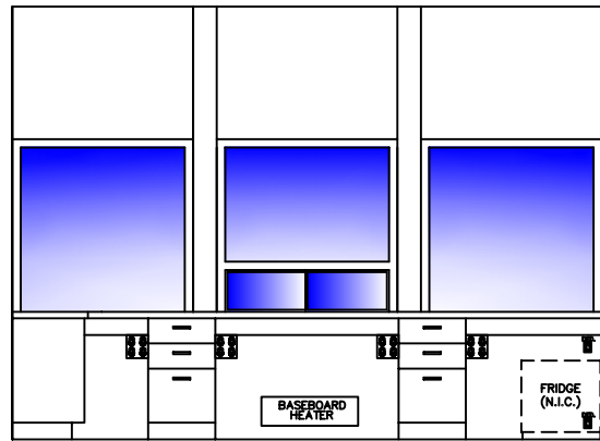
ELEVATION—TICKET BOOTH No.2 SCALE 1:50
