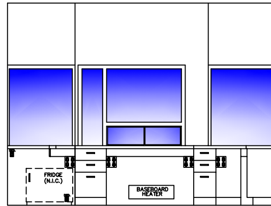
ELEVATION—TICKET BOOTH No.1 SCALE 1:50
