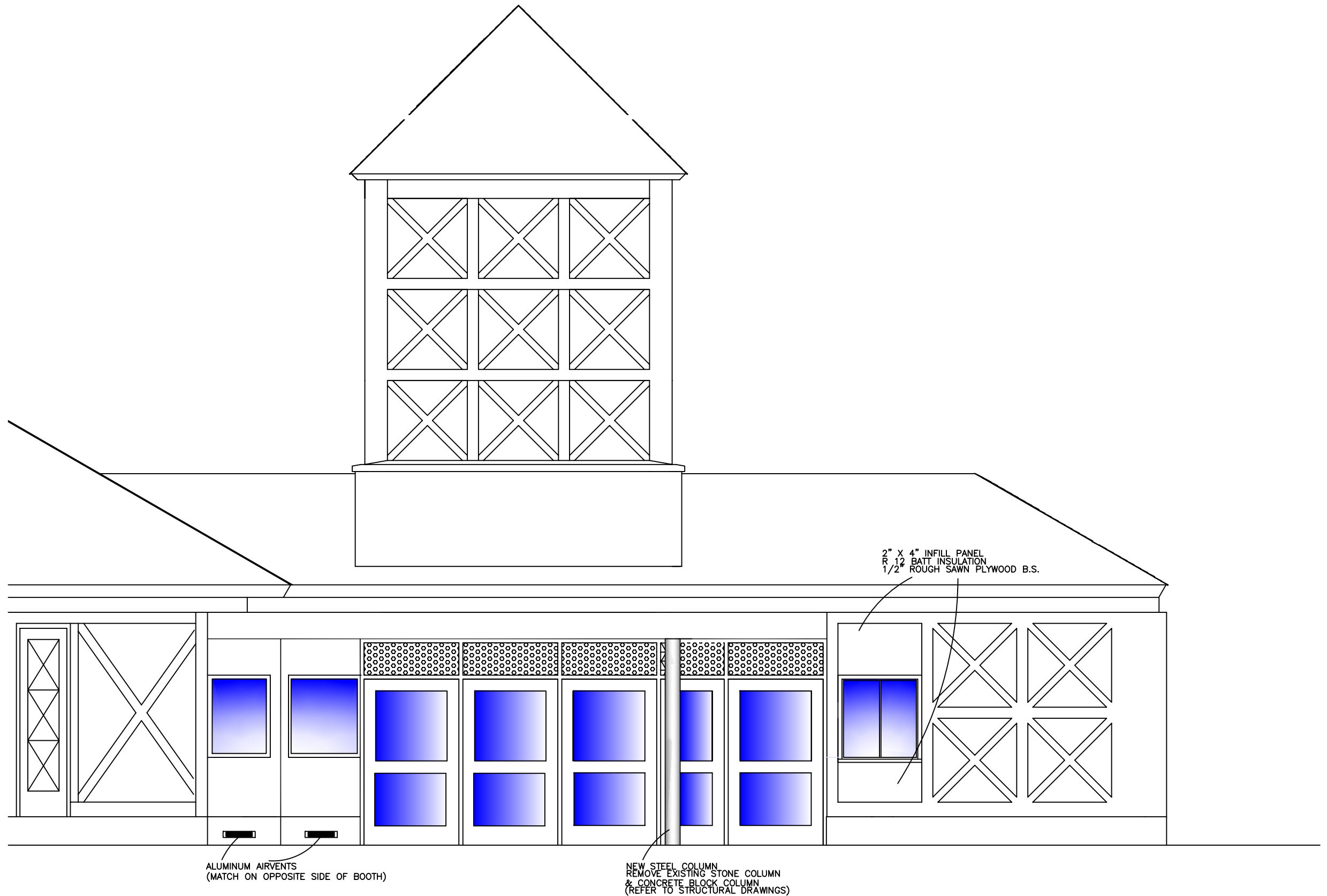
① EAST ELEVATION 2/3 SCALE 1:50
