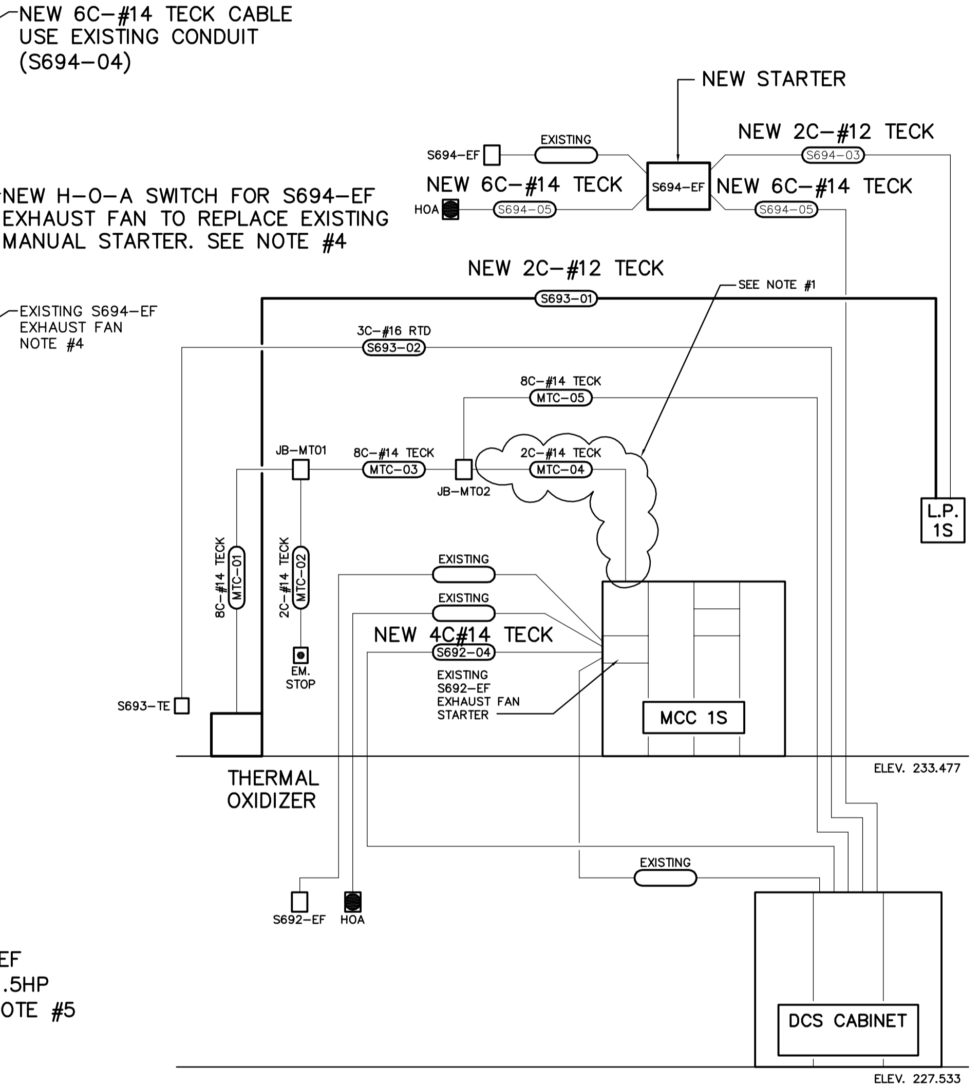
THERMAL OXIDIZER SYSTEM BLOCK DIAGRAM AND CABLE INTERCONNECTION
