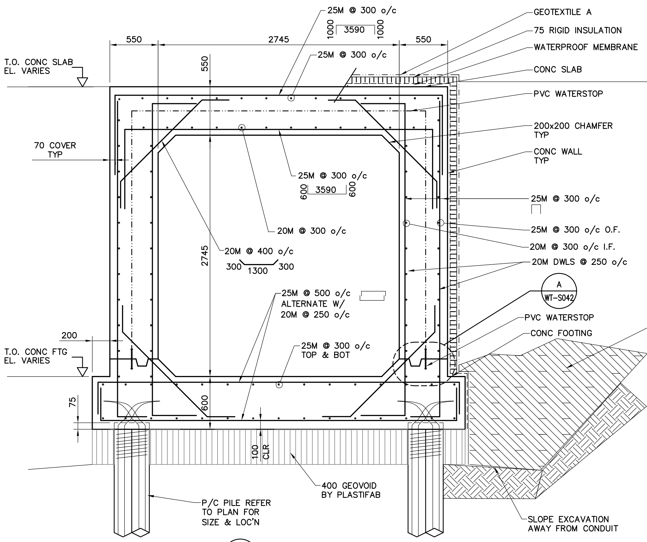
2 SECTION WT-S041 1:25
