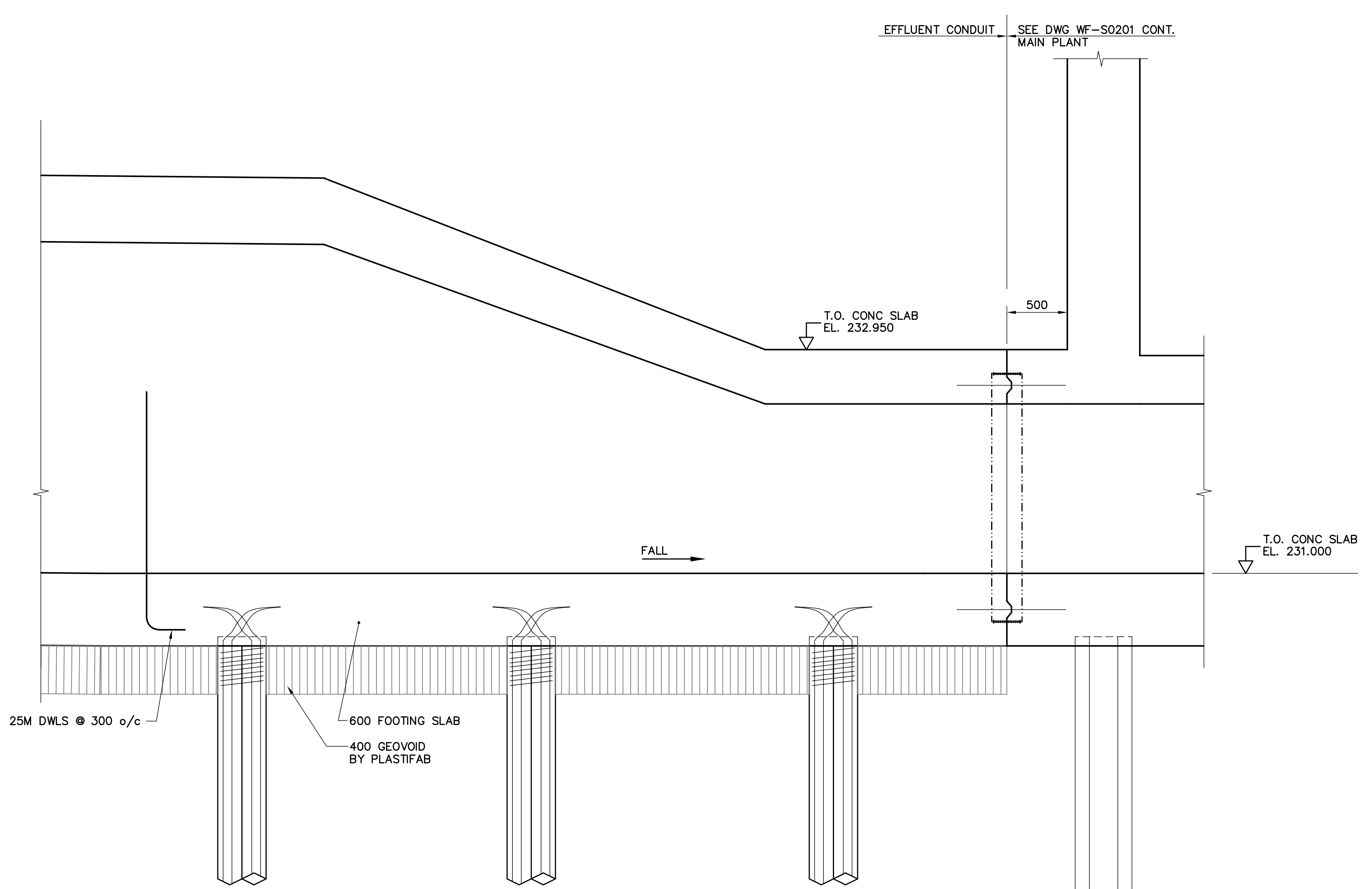
1 SECTION WT-S041 1:25
