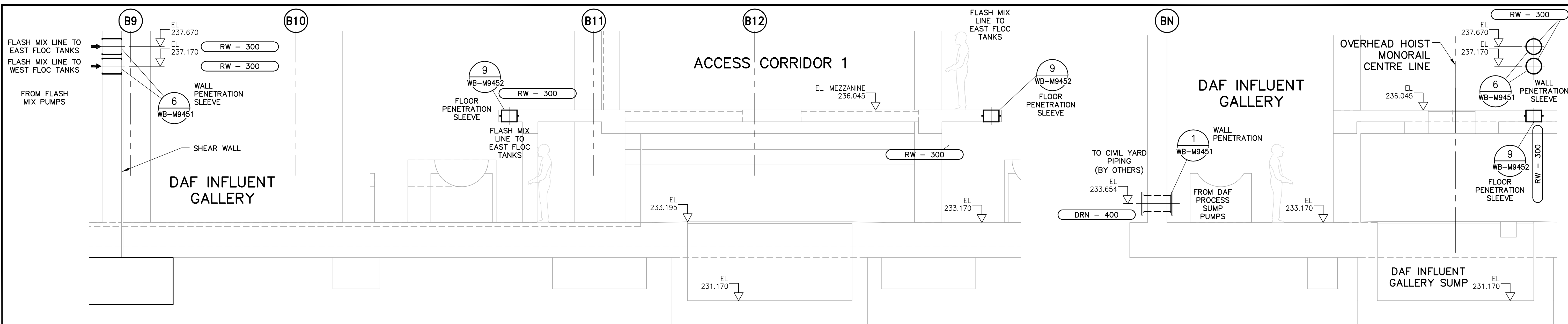
T SECTION - DAF INFLUENT GALLERY SUMP PUMPS WP-M9107 1:50
