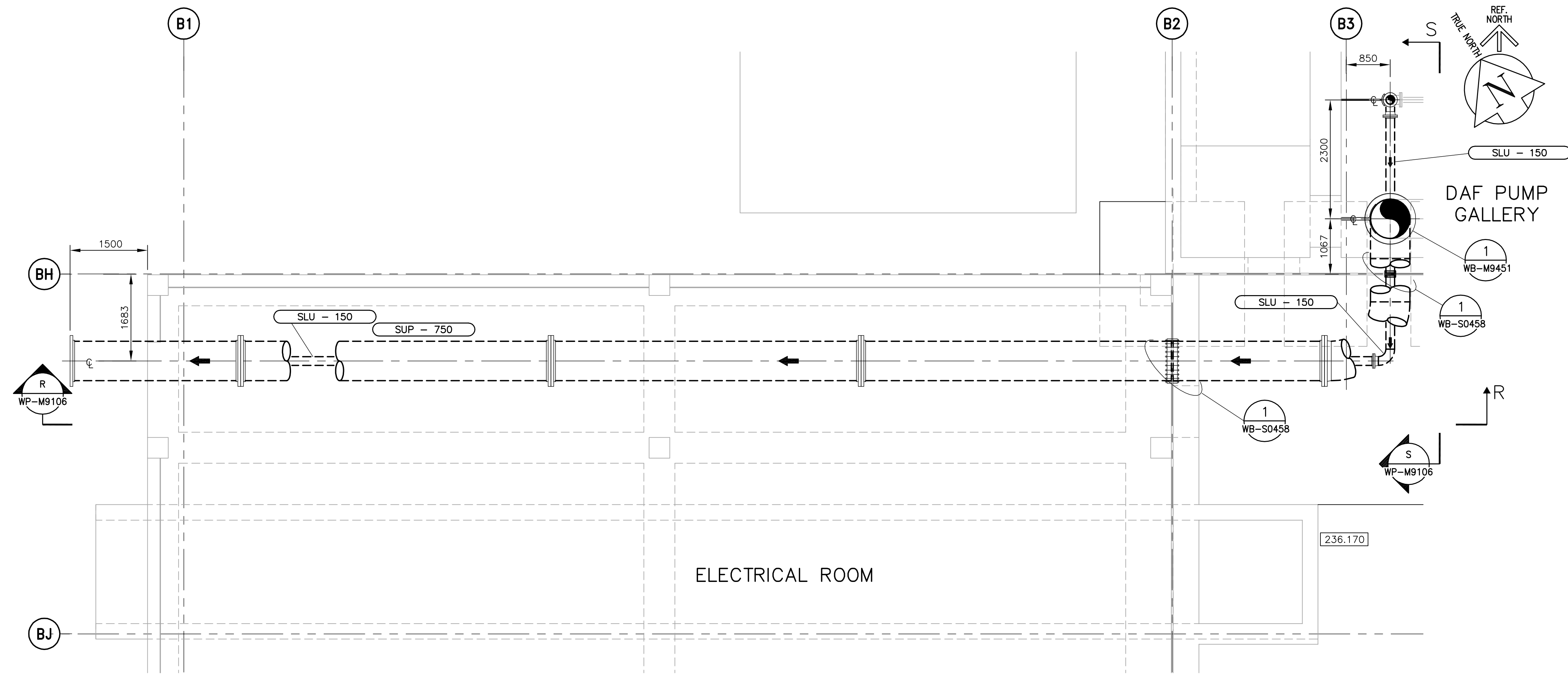
22 FIRST FLOOR PLAN - SUPERNATANT AND SLUDGE LINES WP-M9106 1:50
