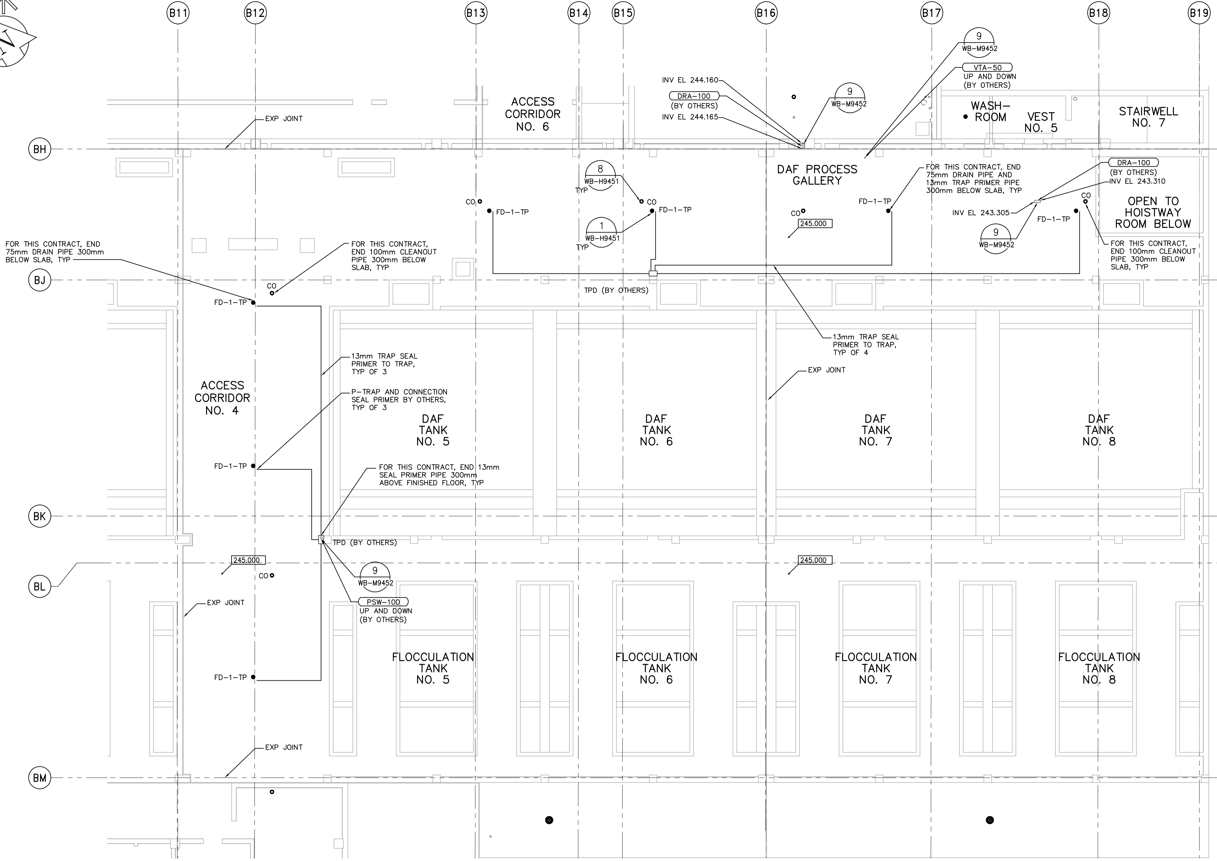
THIRD FLOOR PLAN 1:100
