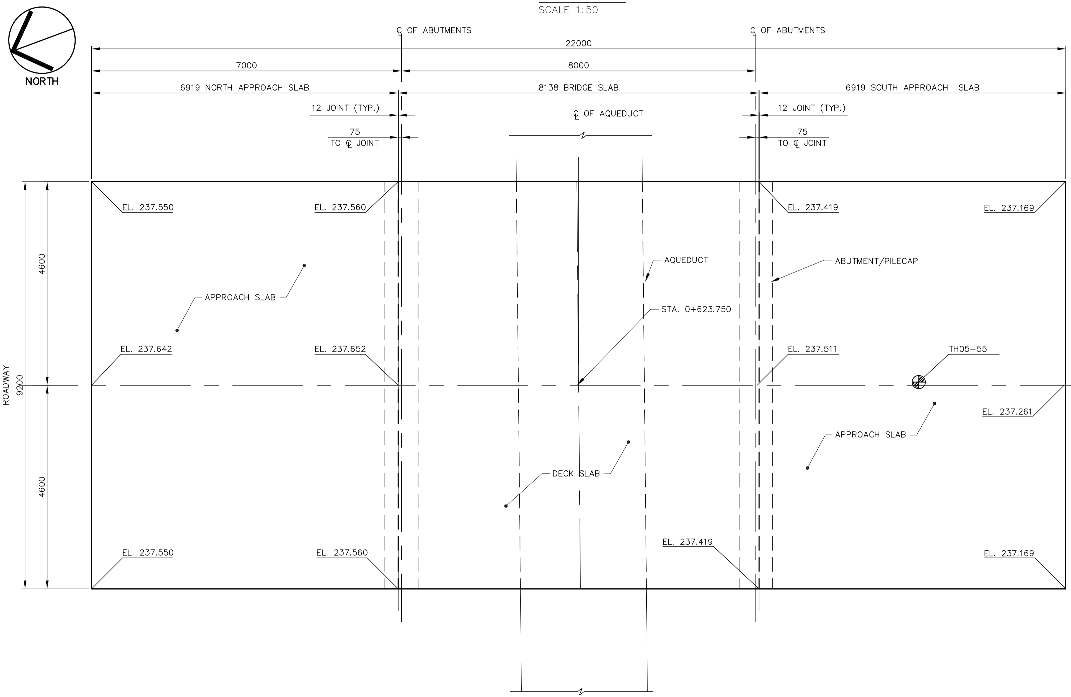
PLAN SCALE 1:50
