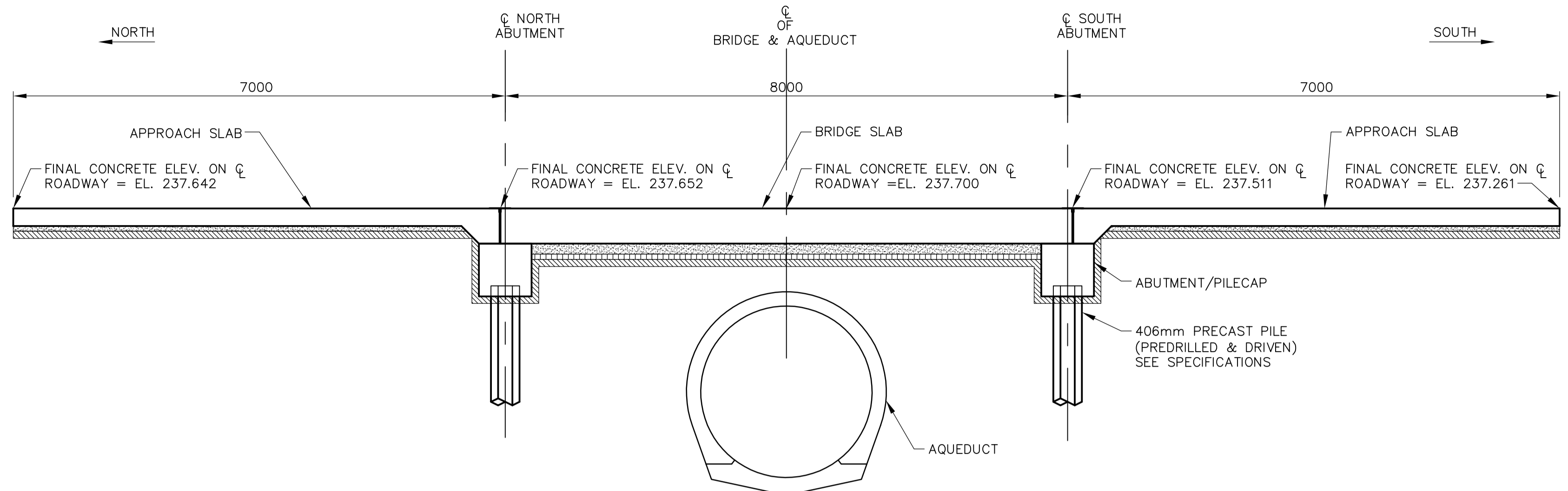
ELEVATION SCALE 1:50
