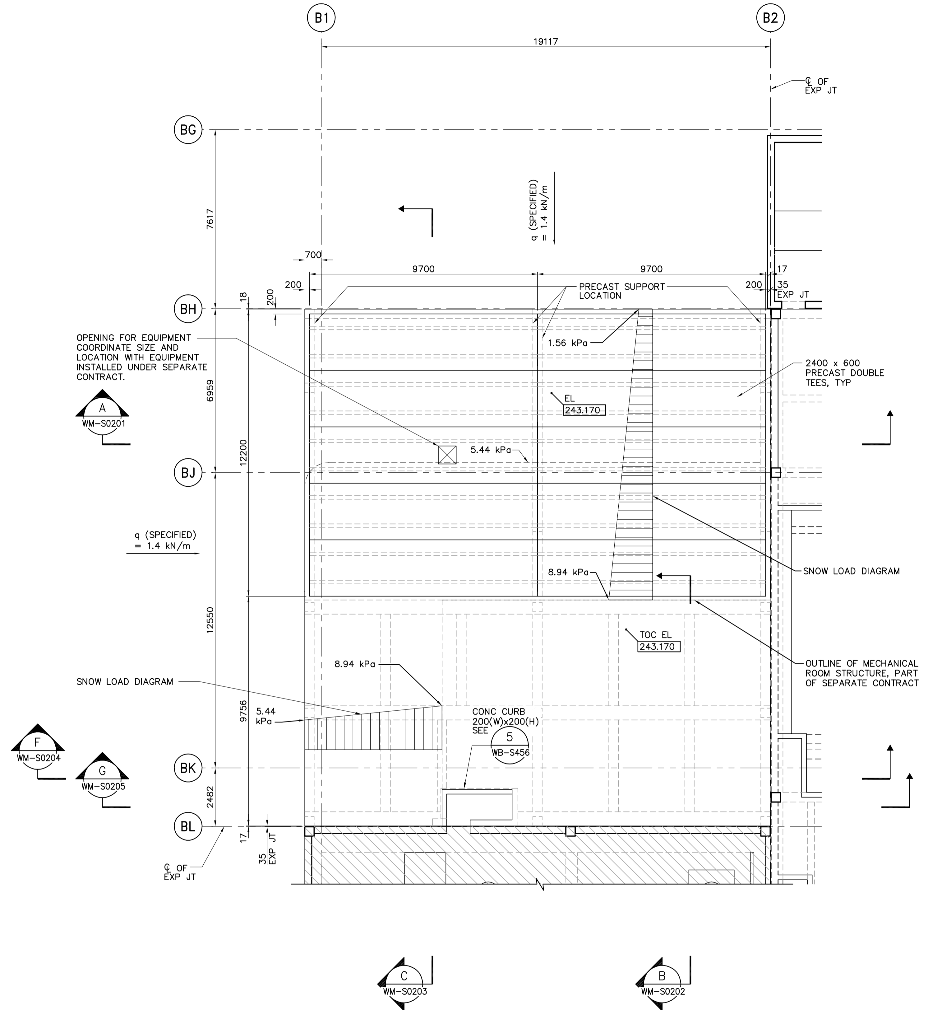
ROOF PLAN 1:100
