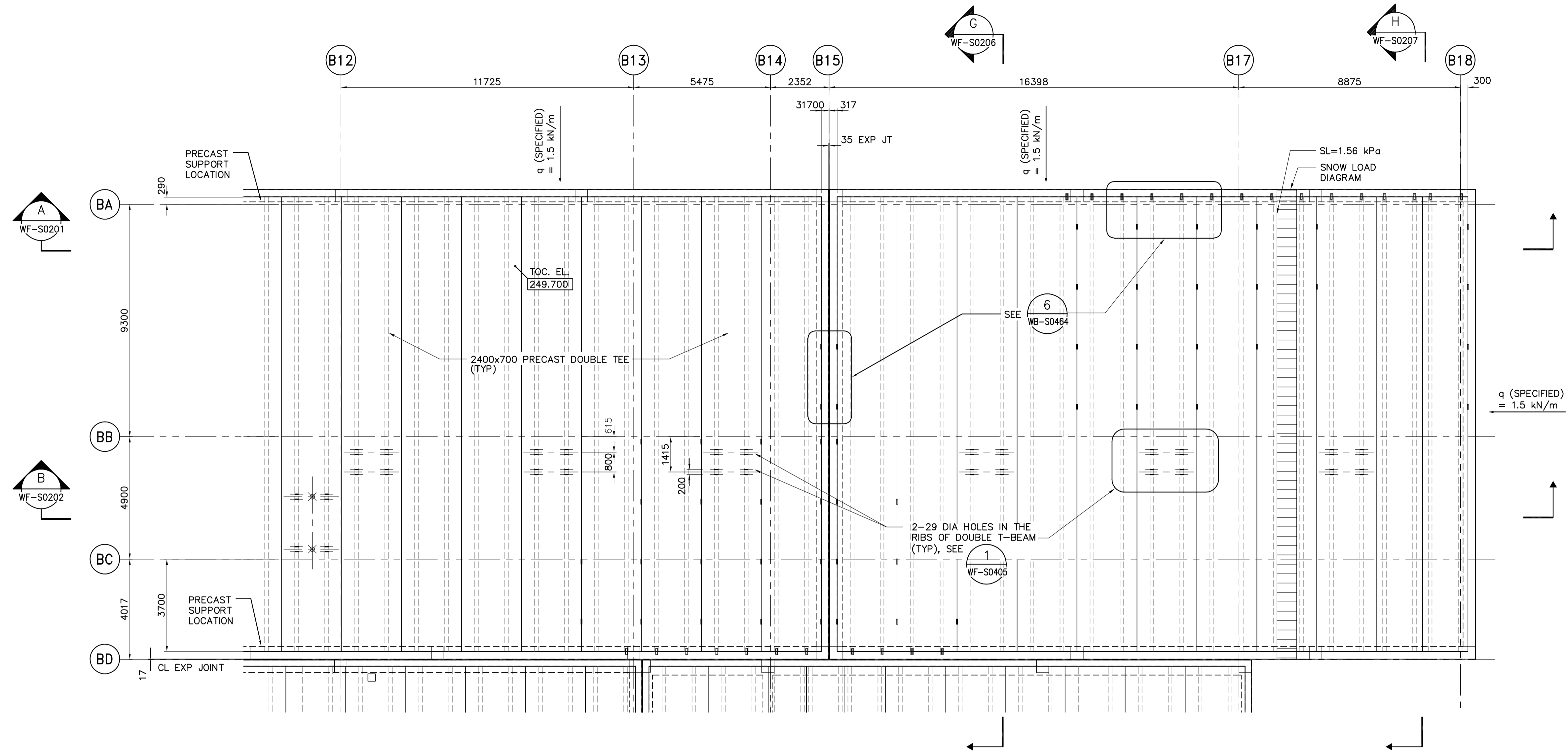
ROOF PLAN 1:100
