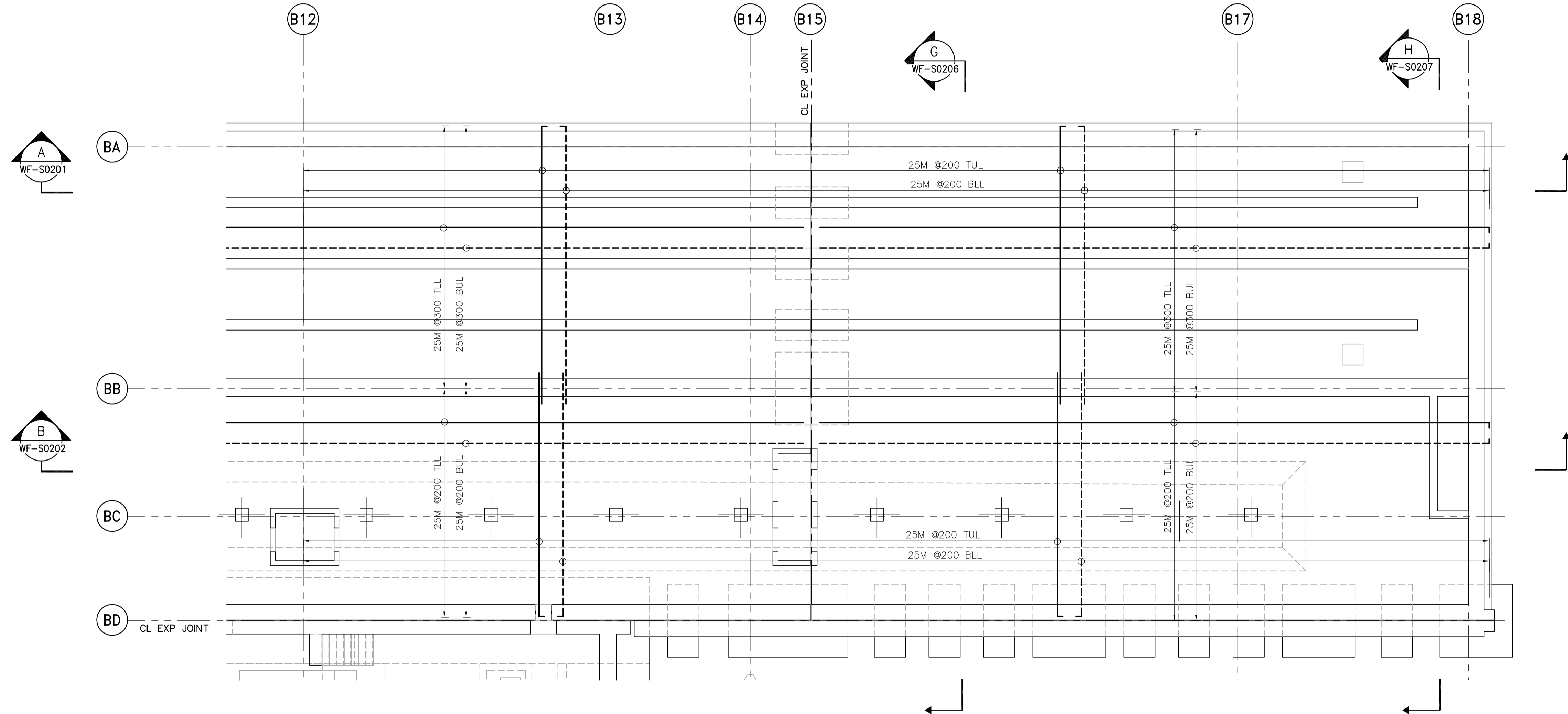
LOWER PLAN AT EL 231.000 1:100
