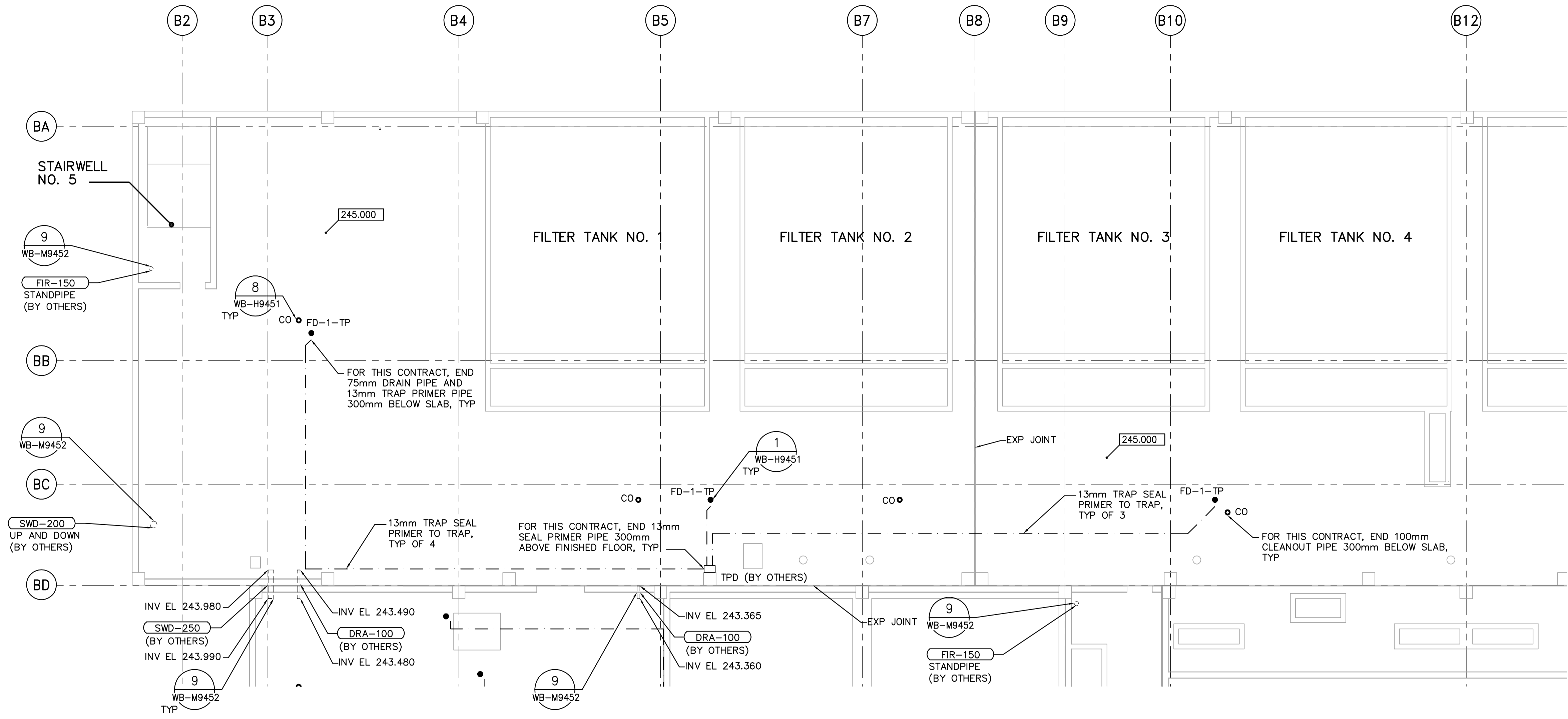
THIRD FLOOR PLAN 1:100
