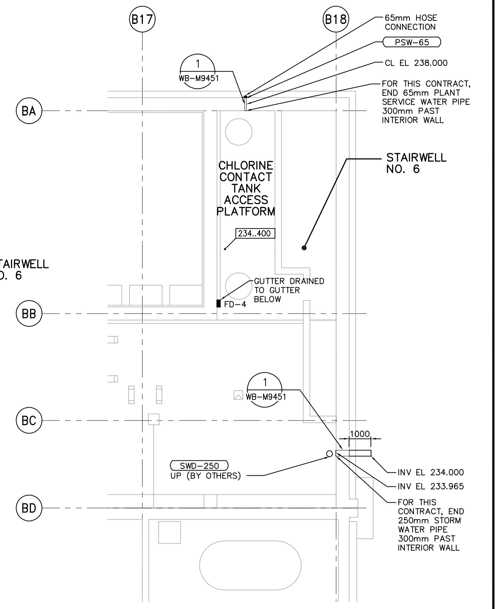
PARTIAL FIRST FLOOR PLAN 1:100
