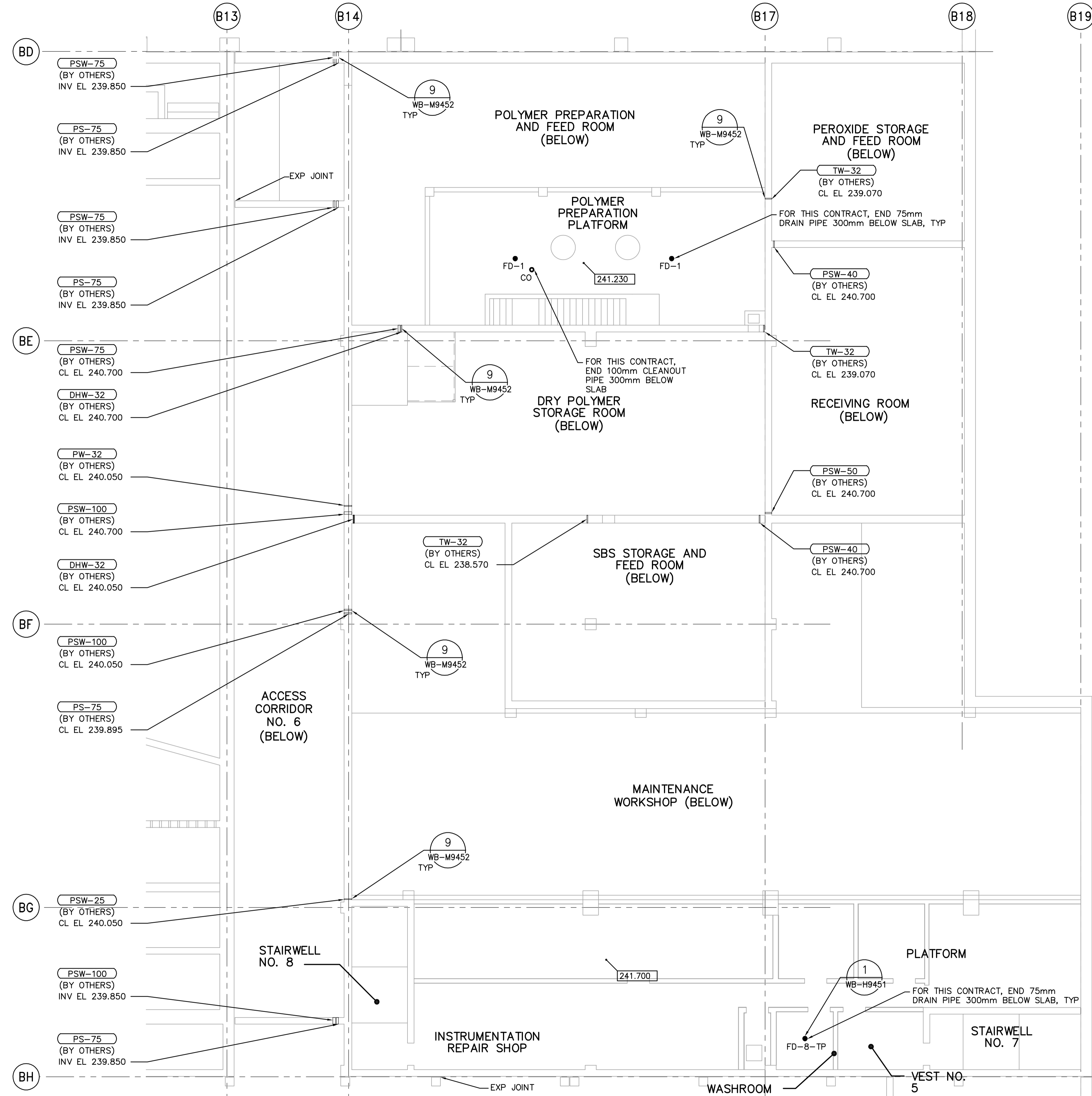
SECOND FLOOR PLAN 1:100
