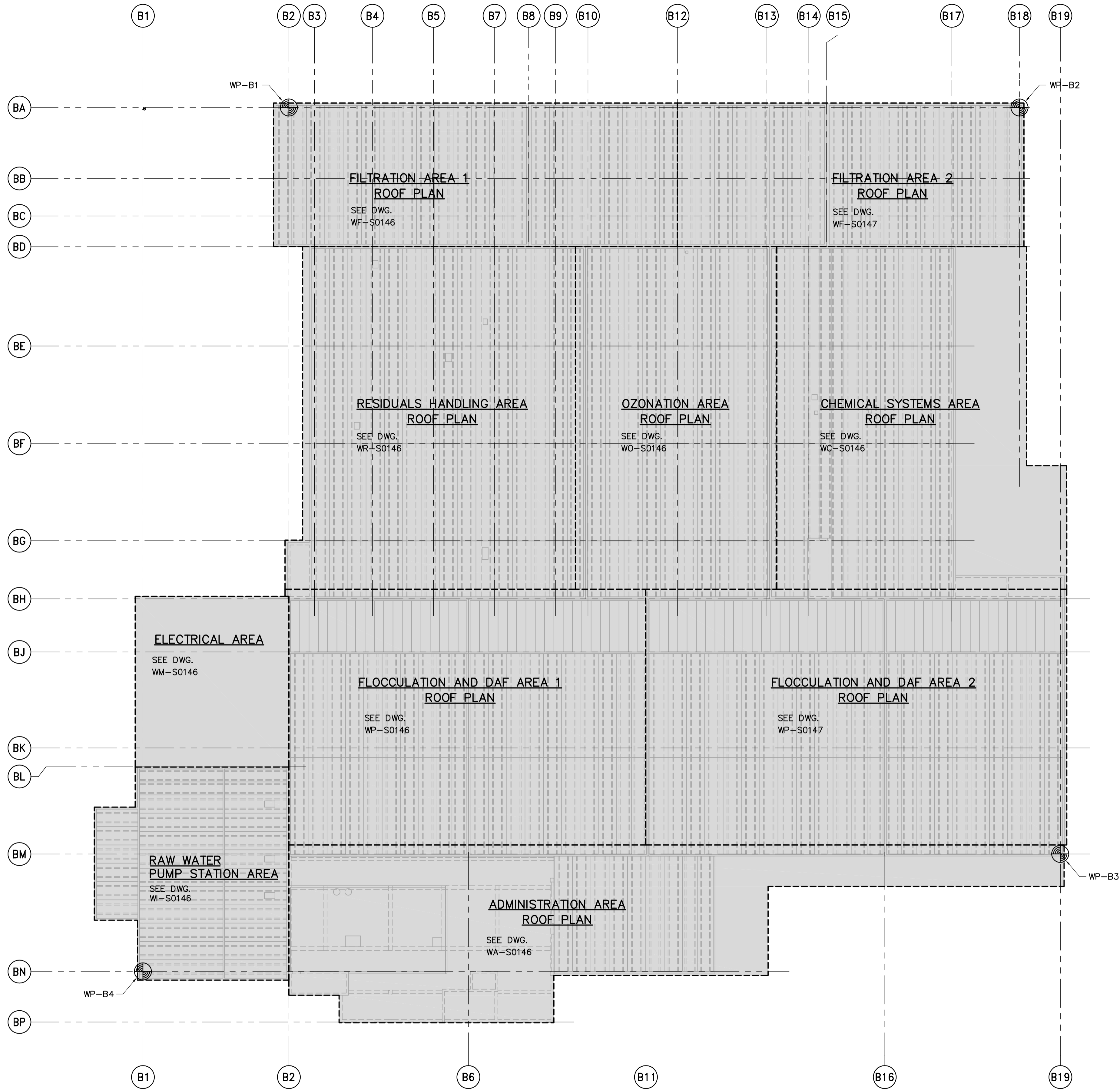
ROOF PLAN 1:300
