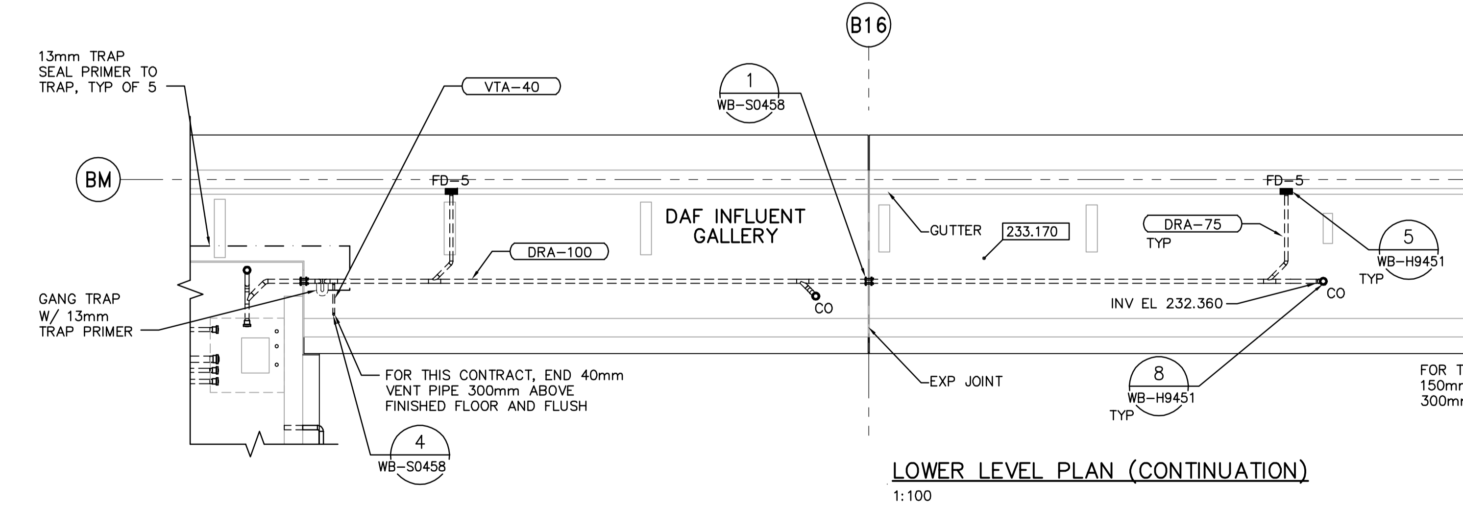
LOWER LEVEL PLAN 1:100
