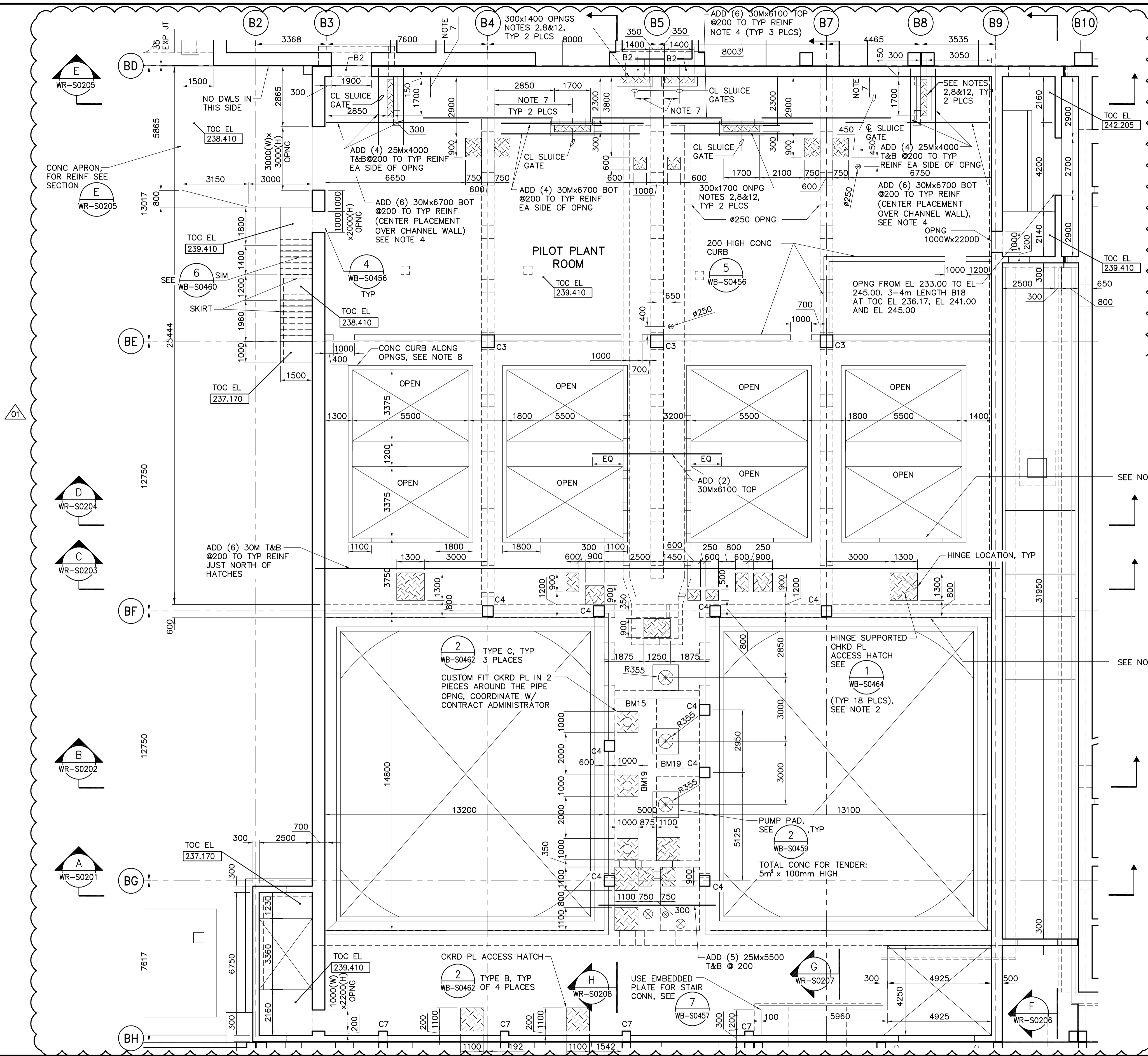
SECOND FLOOR PLAN 1:100
