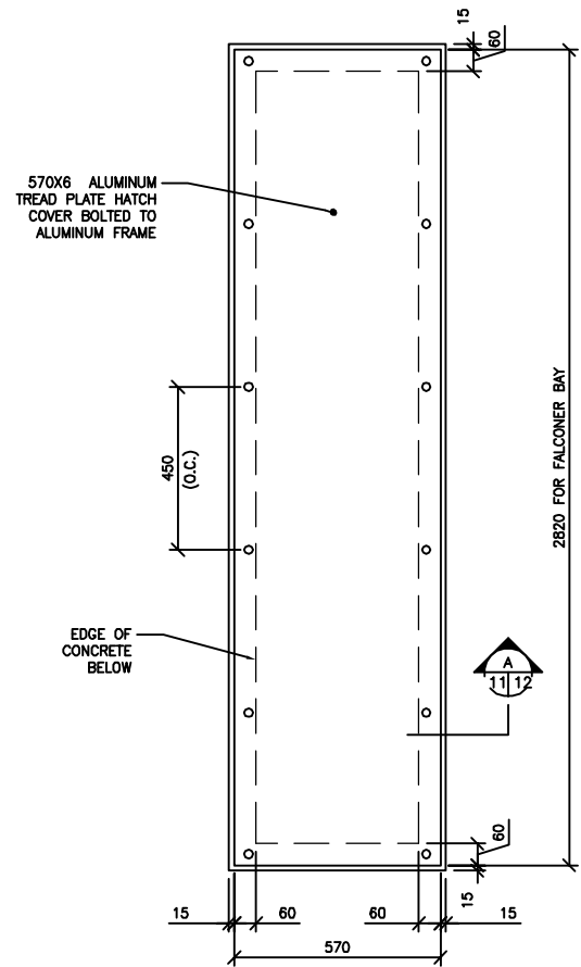
1 DETAIL 1:10
