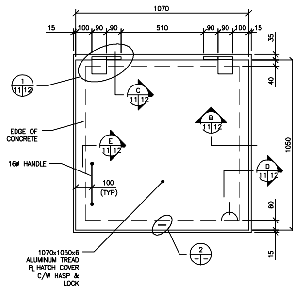
2 DETAIL 1:10
