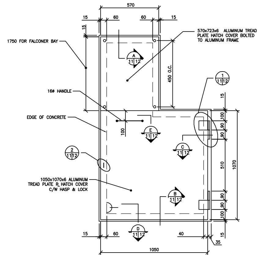
3 DETAIL 1:10
