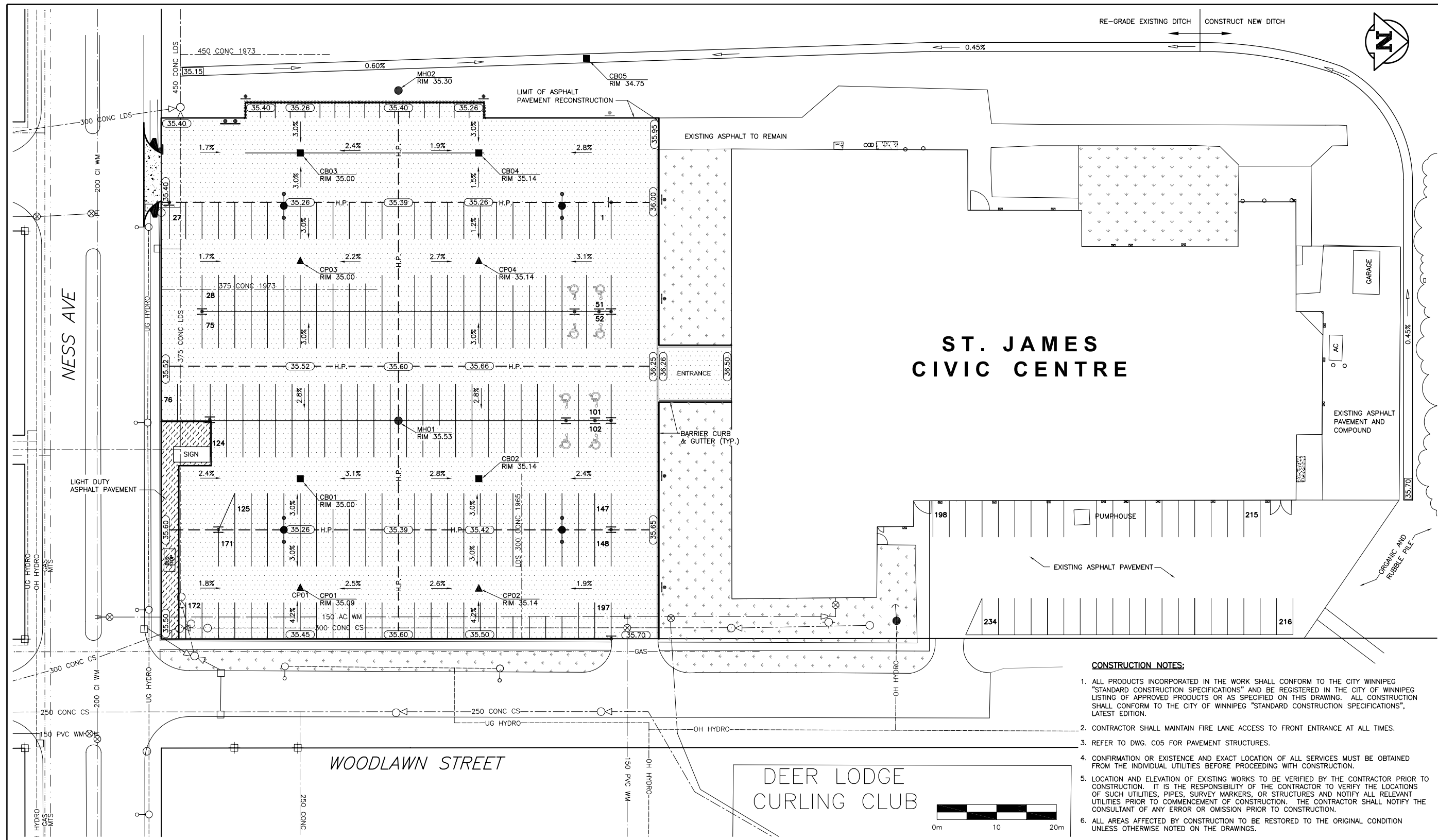
GRADING PLAN SCALE 1:300
