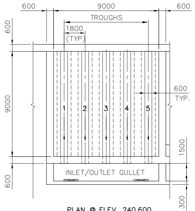
PLAN @ ELEV. 240.600 1:200
