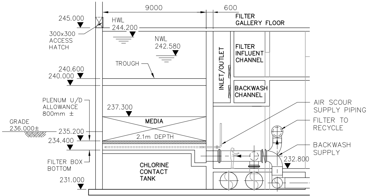
SECTION A 1:200
