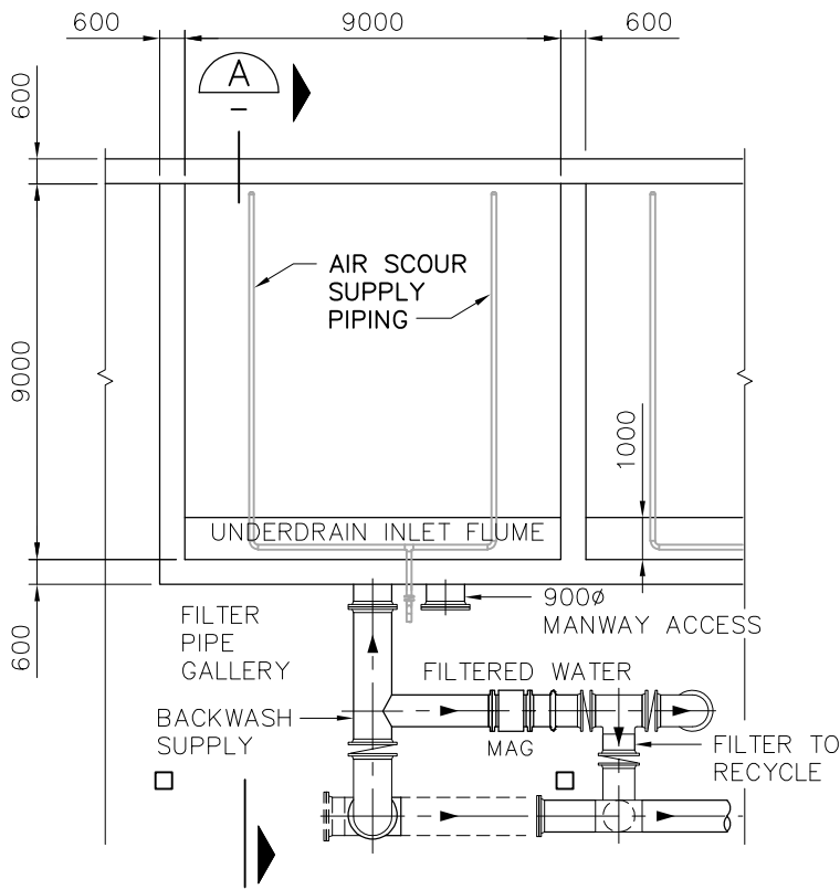
PLAN @ ELEV. 234.400 1:200
