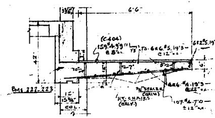
FRONT ENTRANCE CANOPY SECTION 1/8" SCALE
