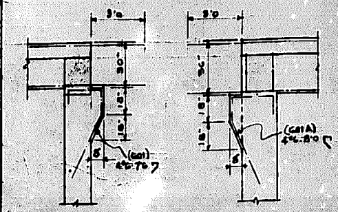
BRACKETS DETAIL COLS. 184 & 185 1/8" SCALE BRACKET DETAIL COLS. 123 & 124 1/8" SCALE
