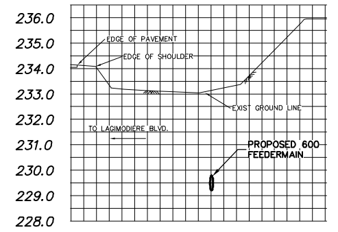
SECTION D-D HORZ. SCALE = 1:500 VERT. SCALE = 1:100
