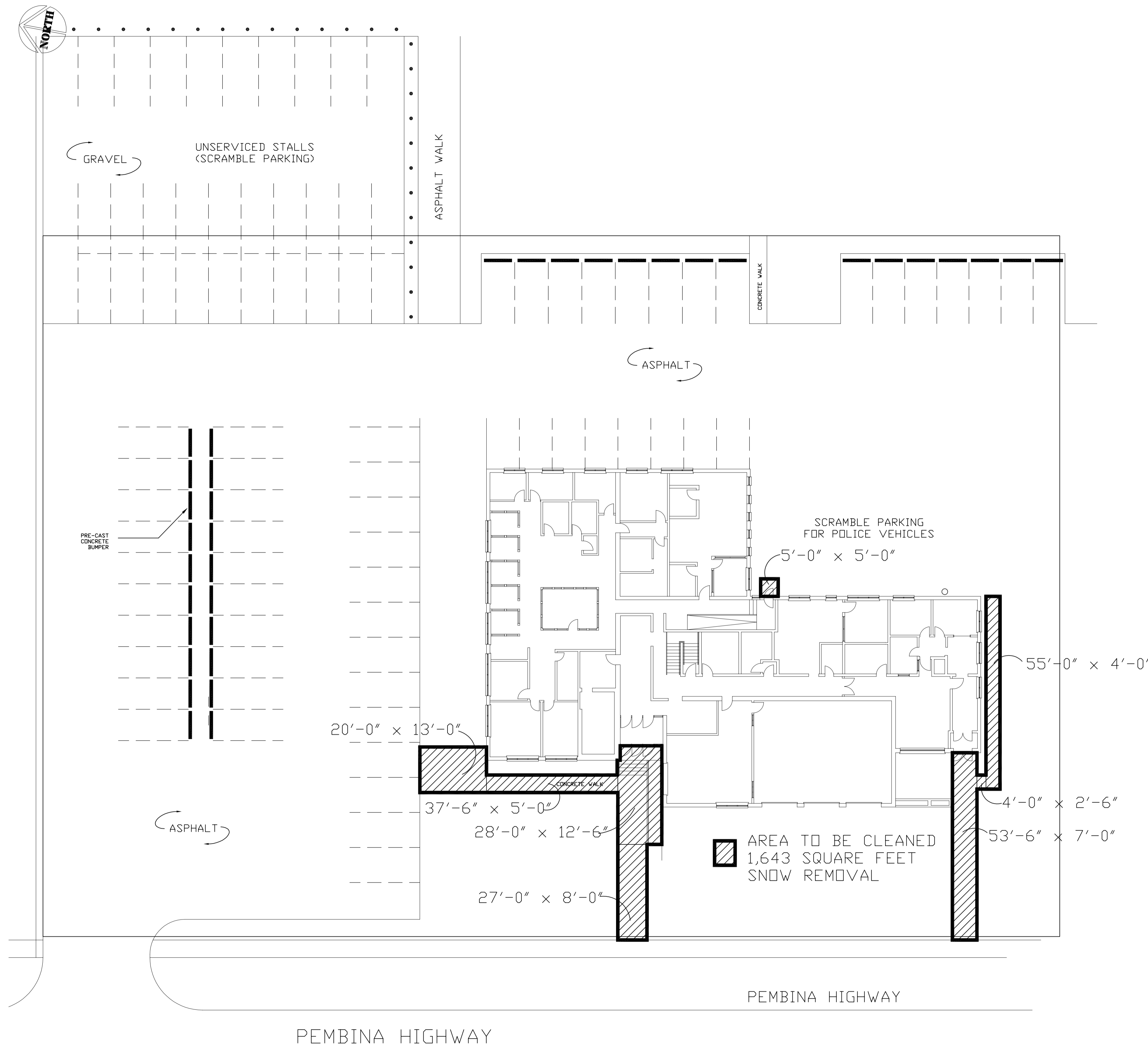
SITE PLAN - SNOW REMOVAL SCALE: 1/16"=1'-0"
