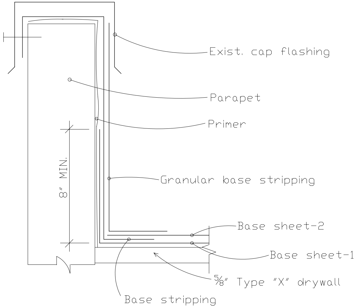
DETAIL "A" - HIGH PARAPET ROOF TERMINATION
