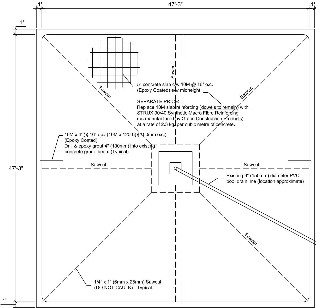
STRUCTURAL PLAN VIEW SCALE: 1/8" = 1' - 0"
