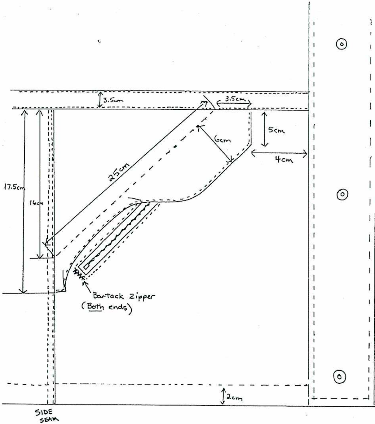
POCKET DETAIL SIZE: MEDIUM REGULAR
