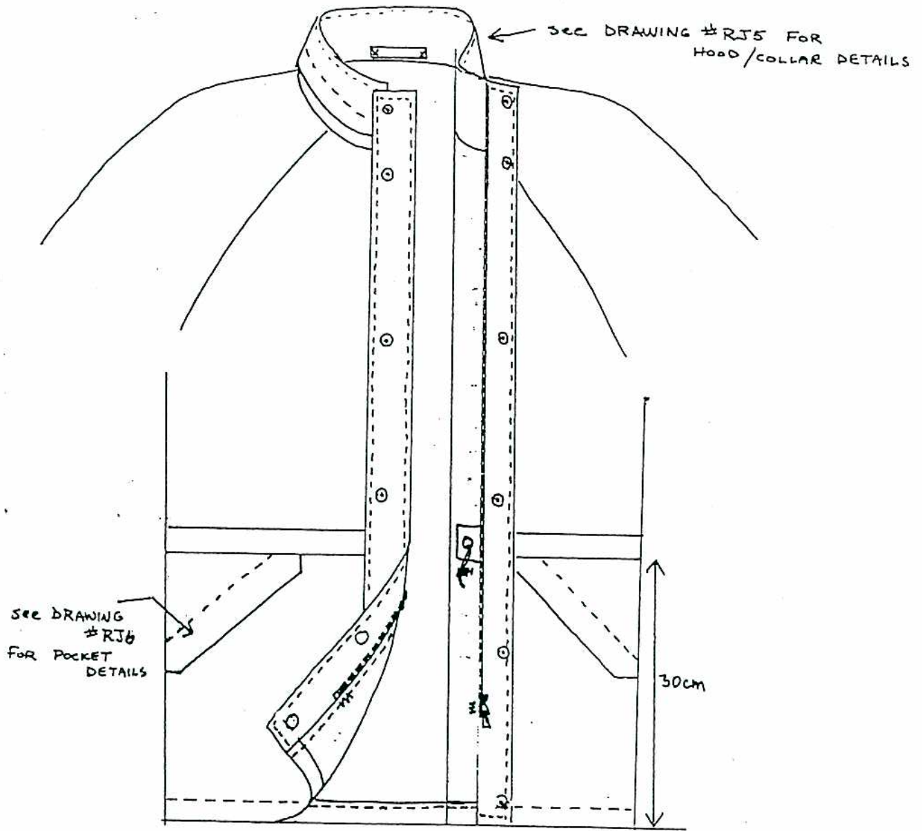
DOUBLE FLAP DETAIL
