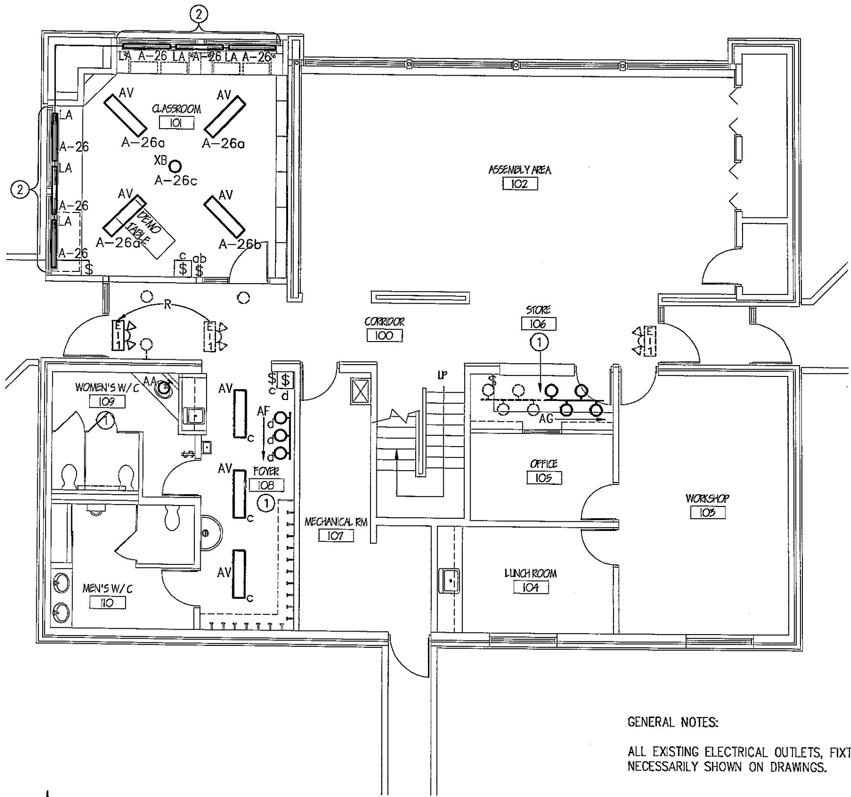
FLOOR PLAN - LIGHTING SCALE: 1/8" = 1'-0"
