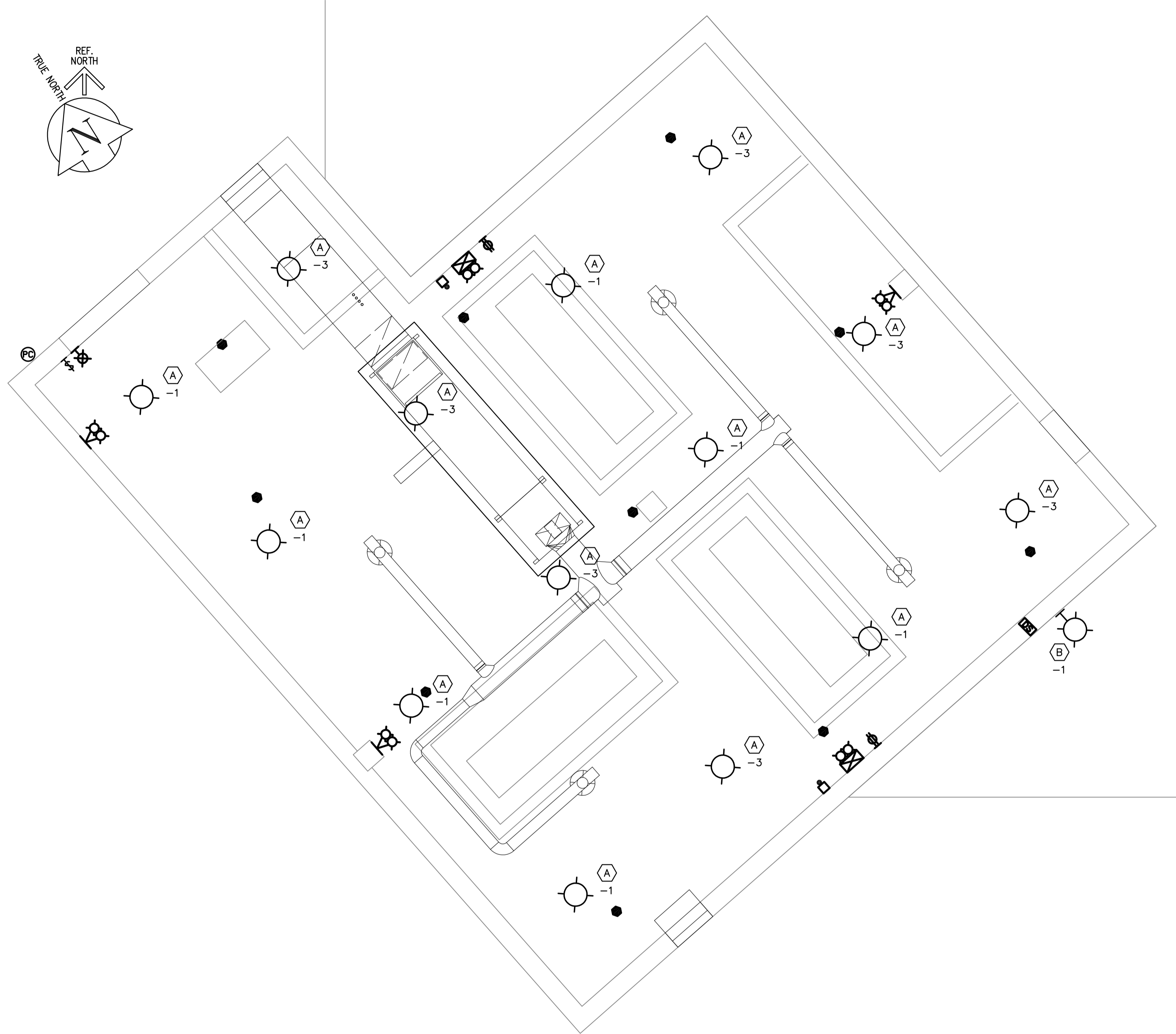
MAIN FLOOR POWER PLAN 1:100
