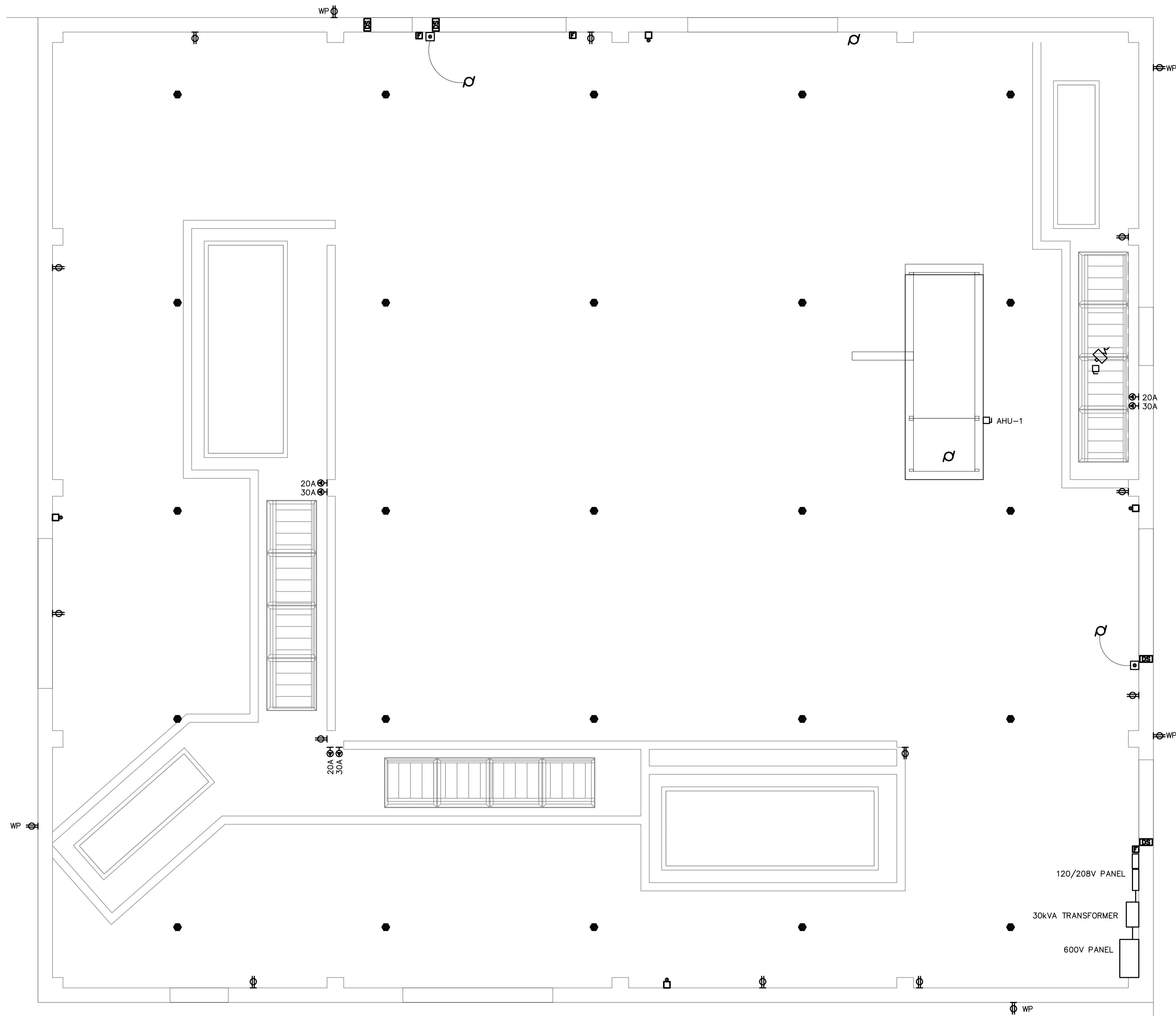
MAIN FLOOR POWER PLAN 1:50
