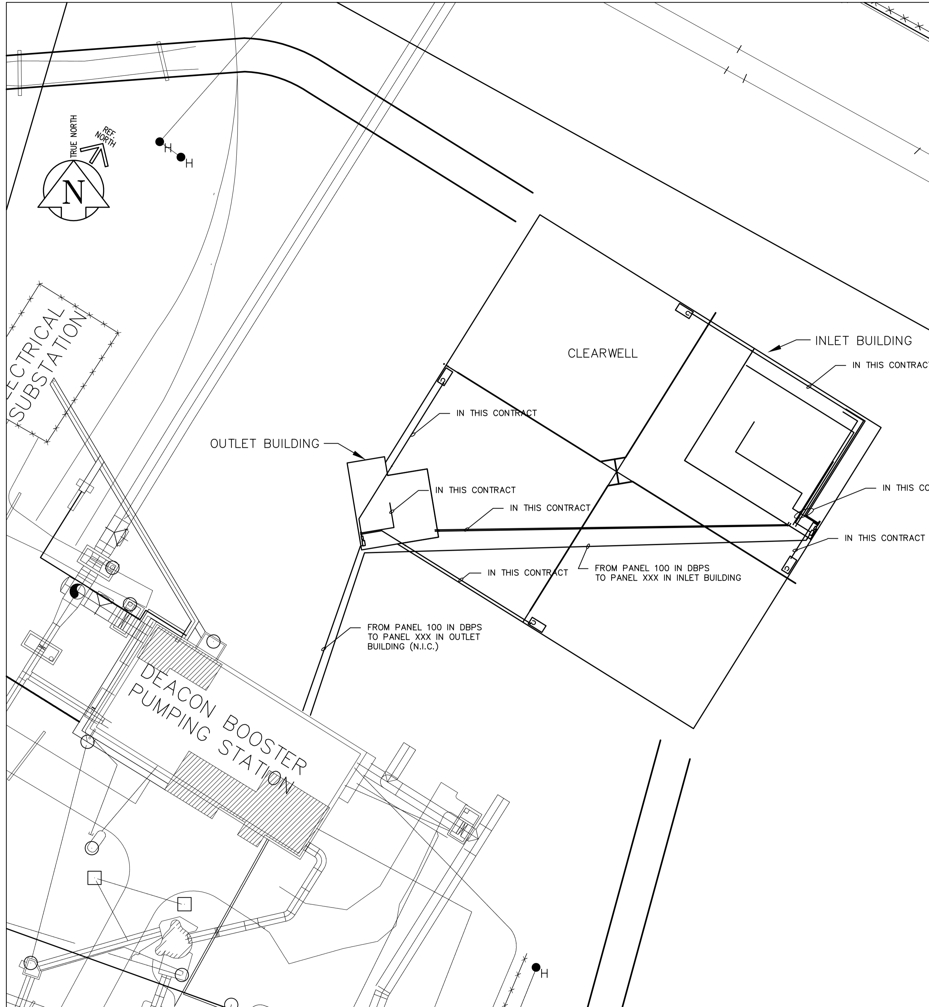
PARTIAL ELECTRICAL SITE PLAN 1:400
