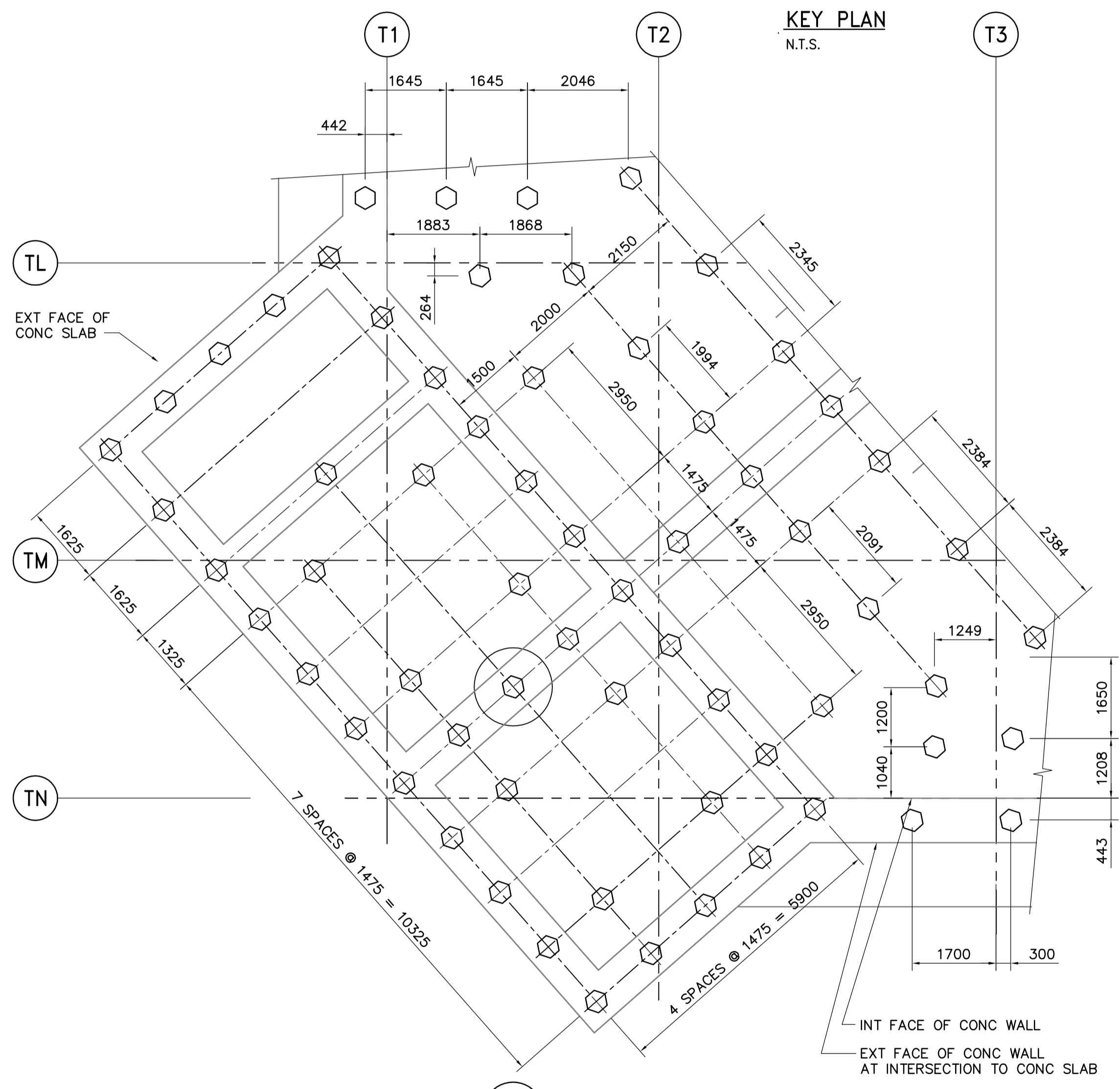
DETAIL 1:75
