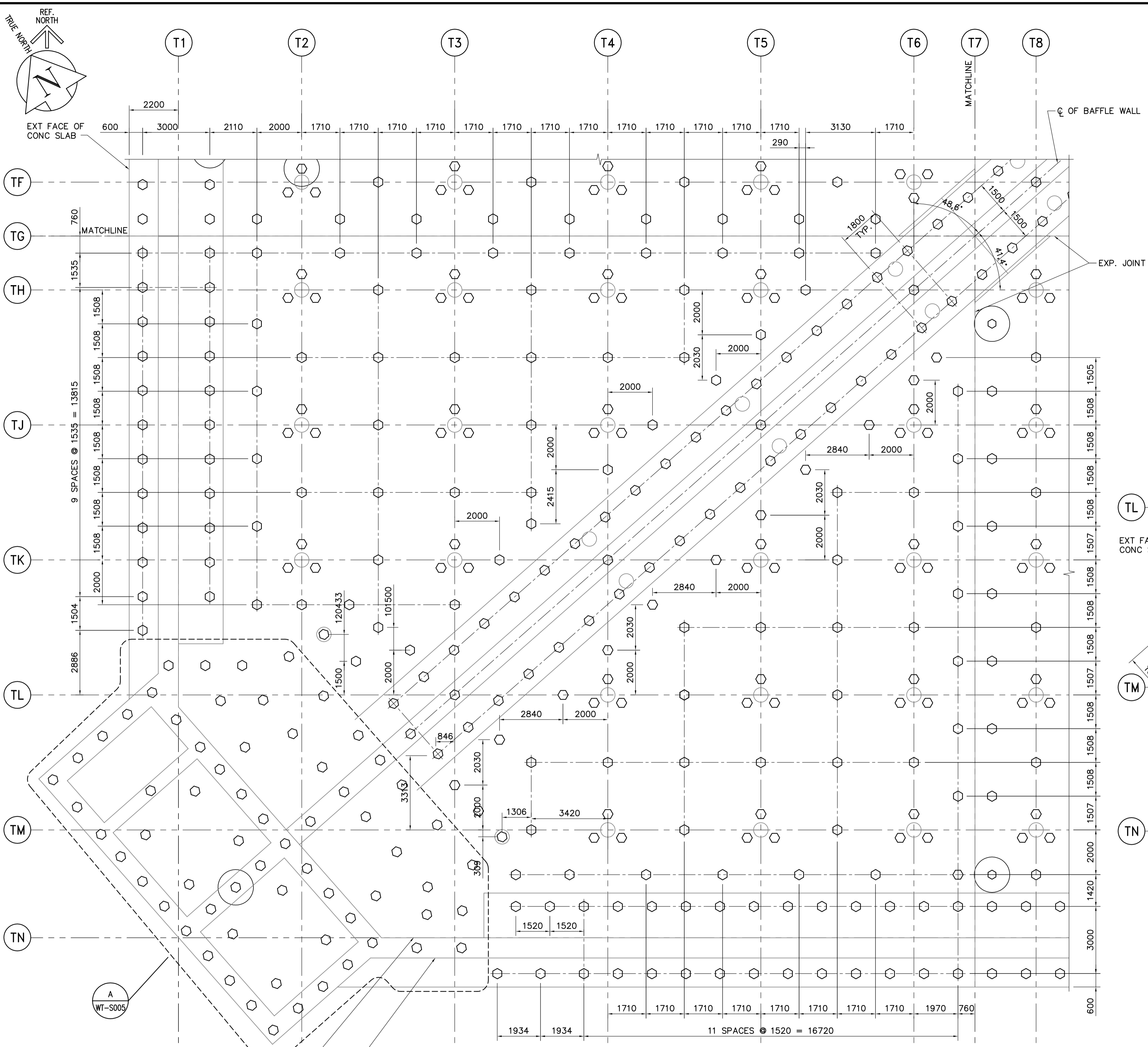
PARTIAL PILING PLAN 1:100
