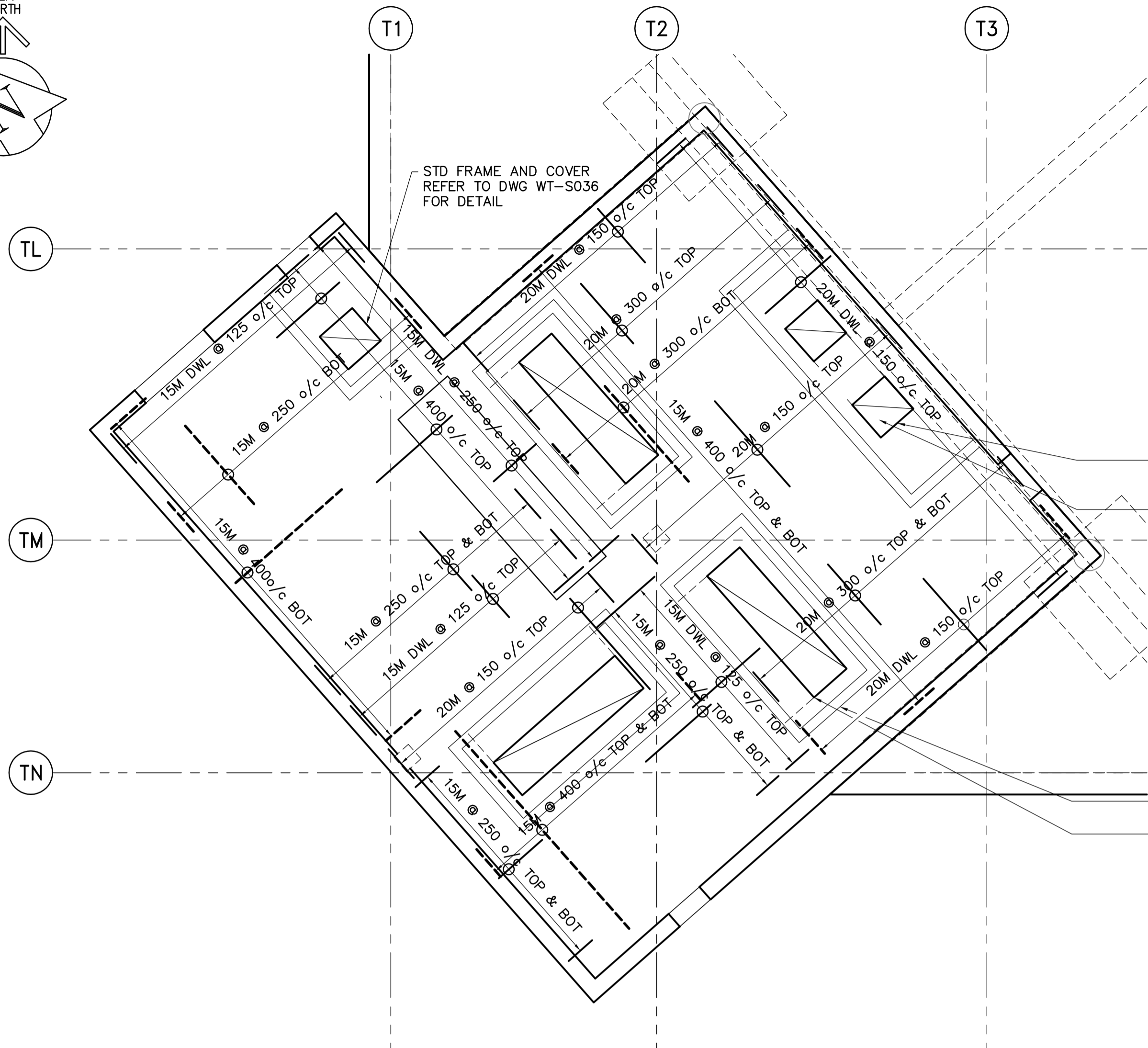
MAIN FLOOR REINFORCING PLAN 1:75
