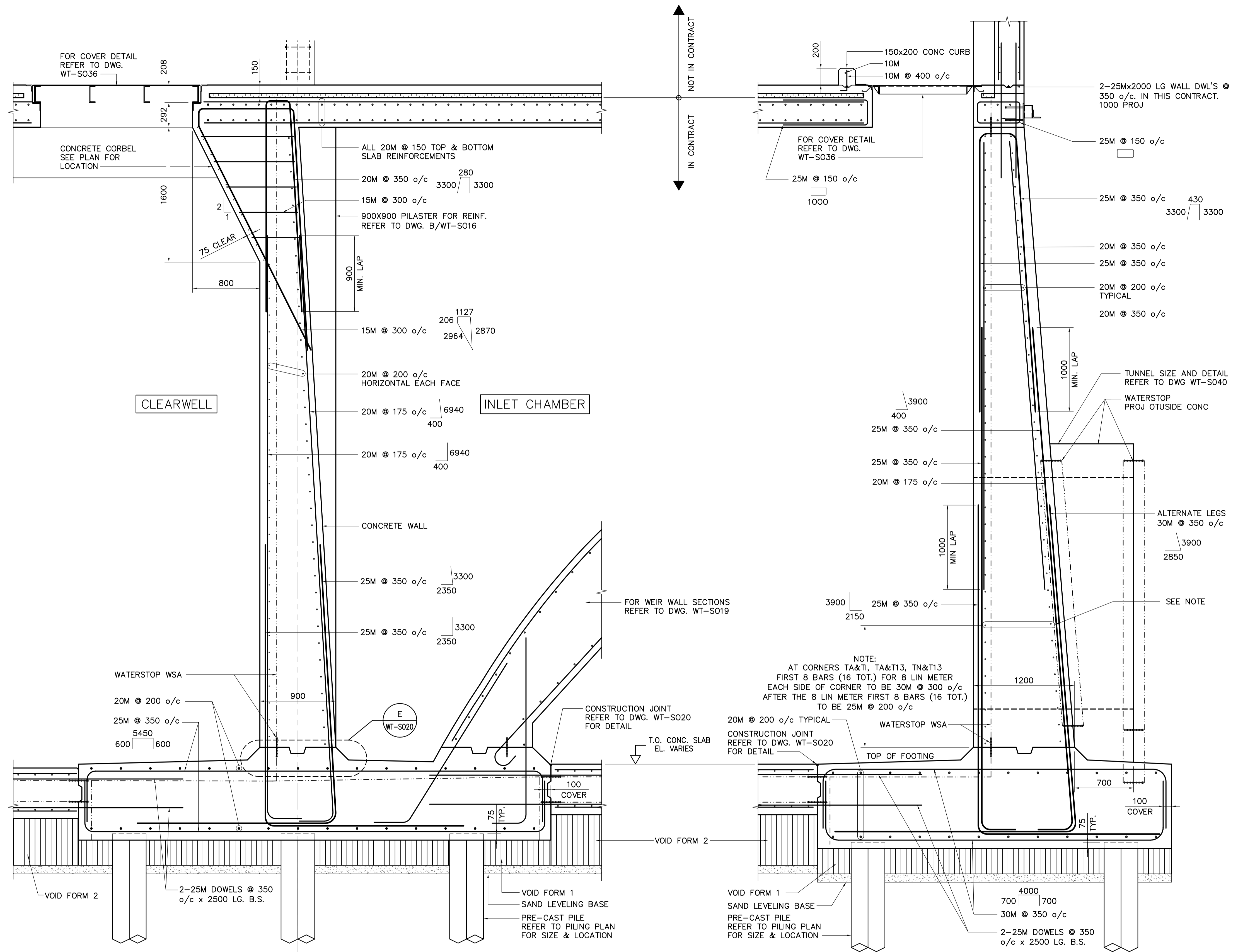
G DETAIL WT-S014 1:25
