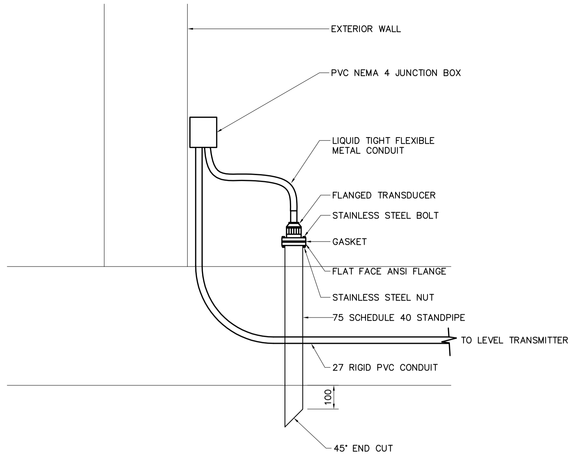
1 DETAIL 1001 SCALE NTS
